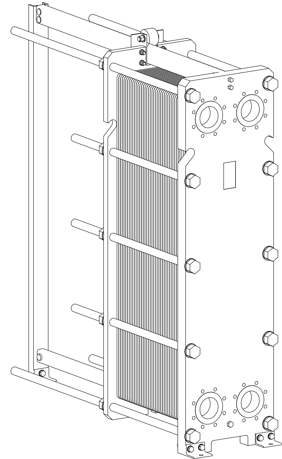
Isometric view
