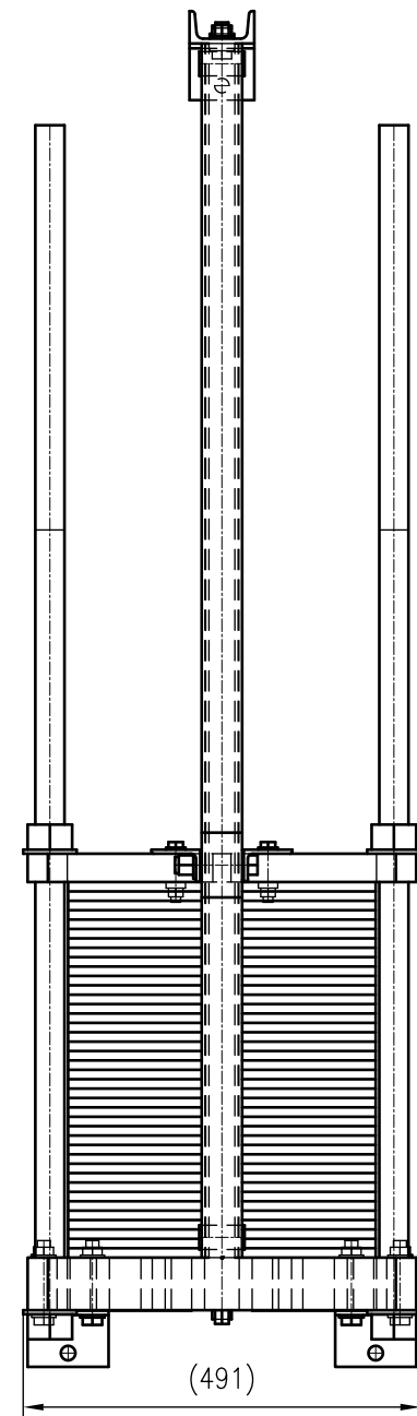
Top view
