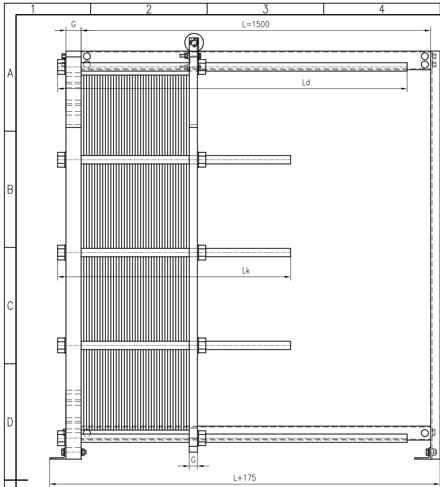
Side view
