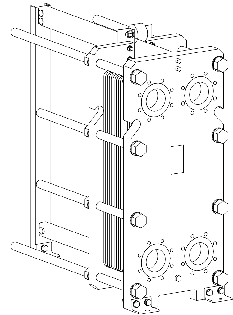
Isometric view
