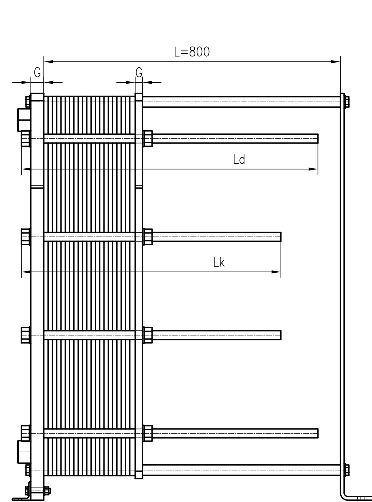
Side view
