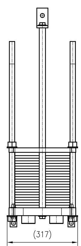
Top view
