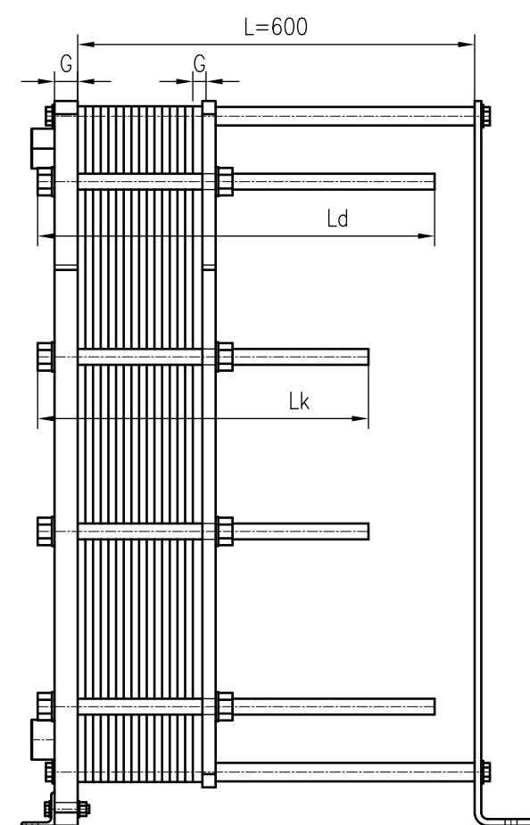
Side view
