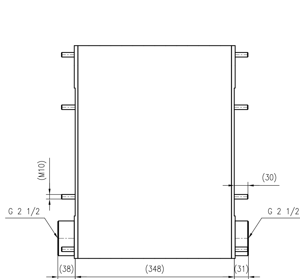
Side view
