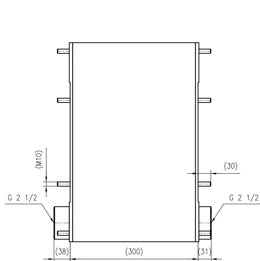
Side view
