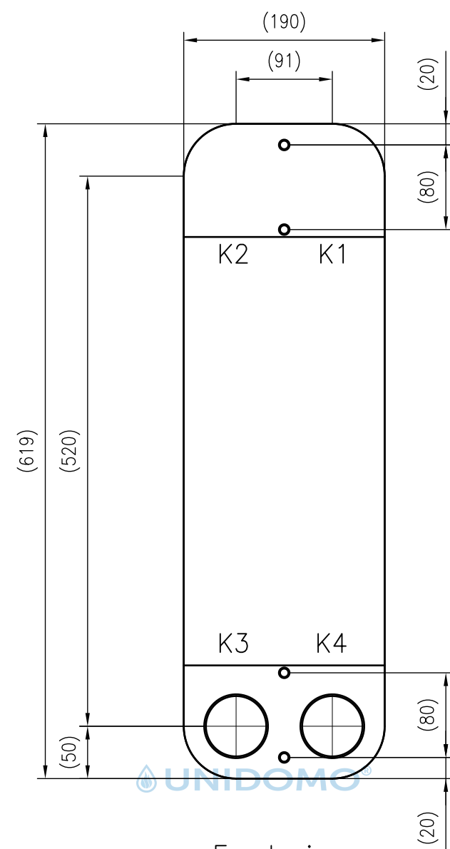
Front view
