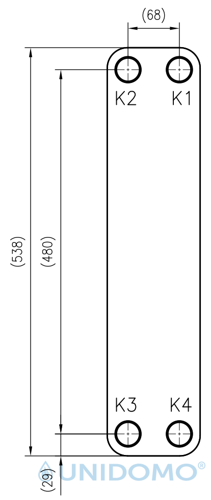
Front view
