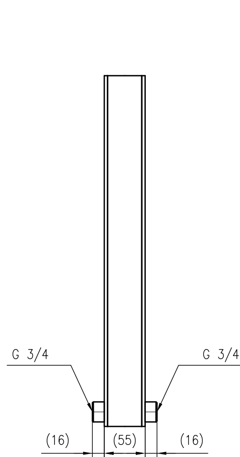
Side view
