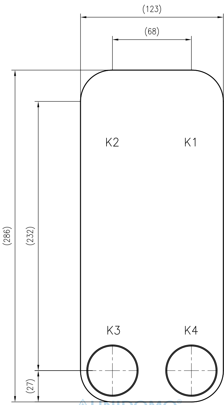
Front view
