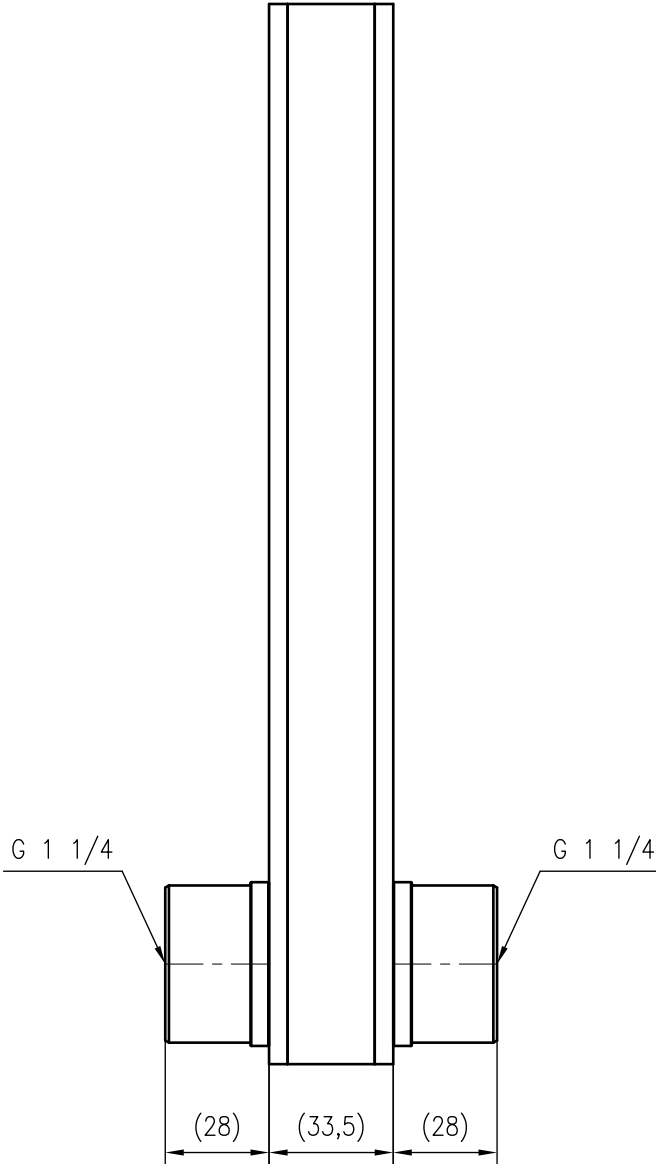
Side view
