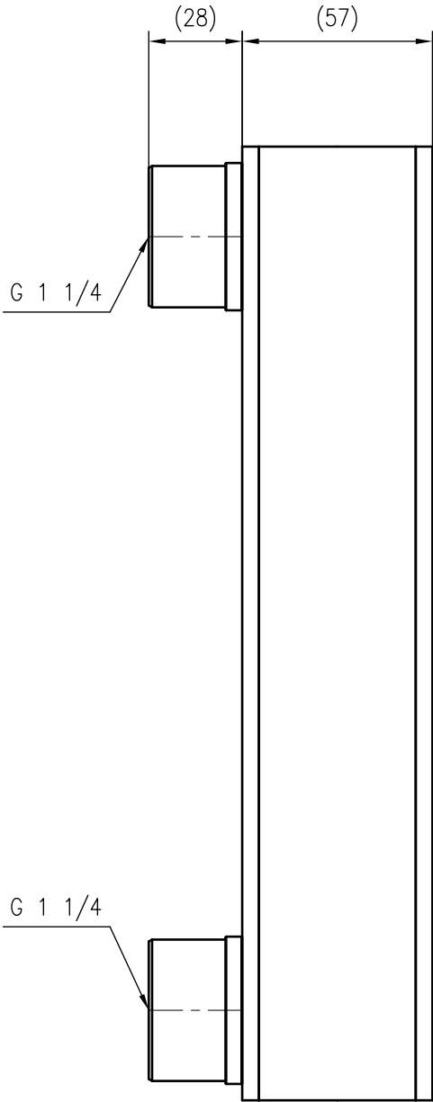
Side view
