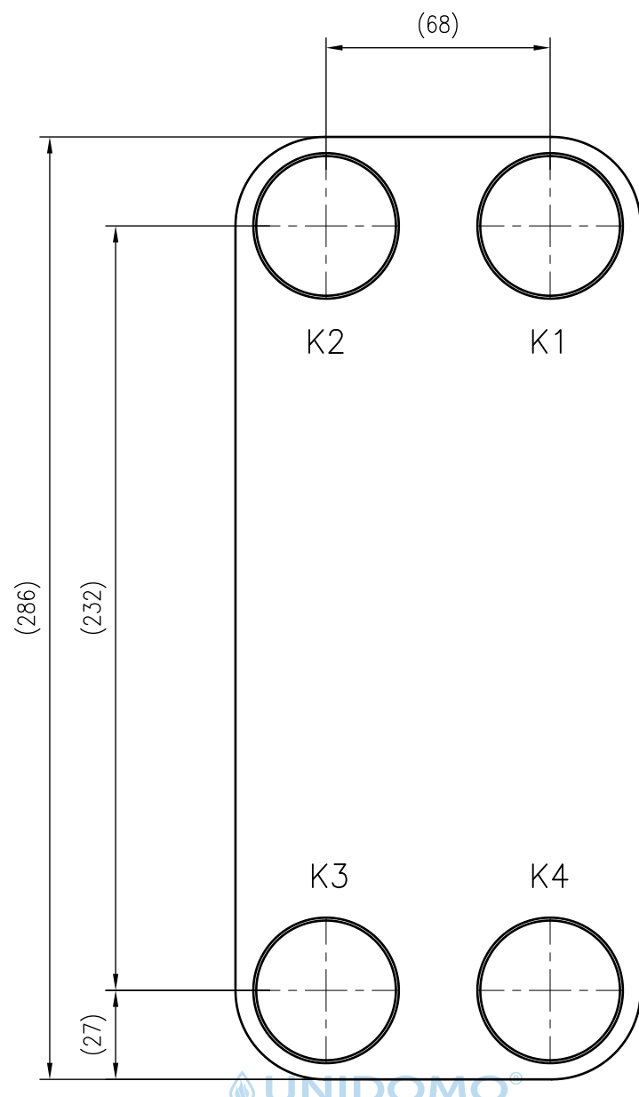
Front view
