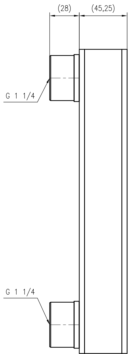
Side view
