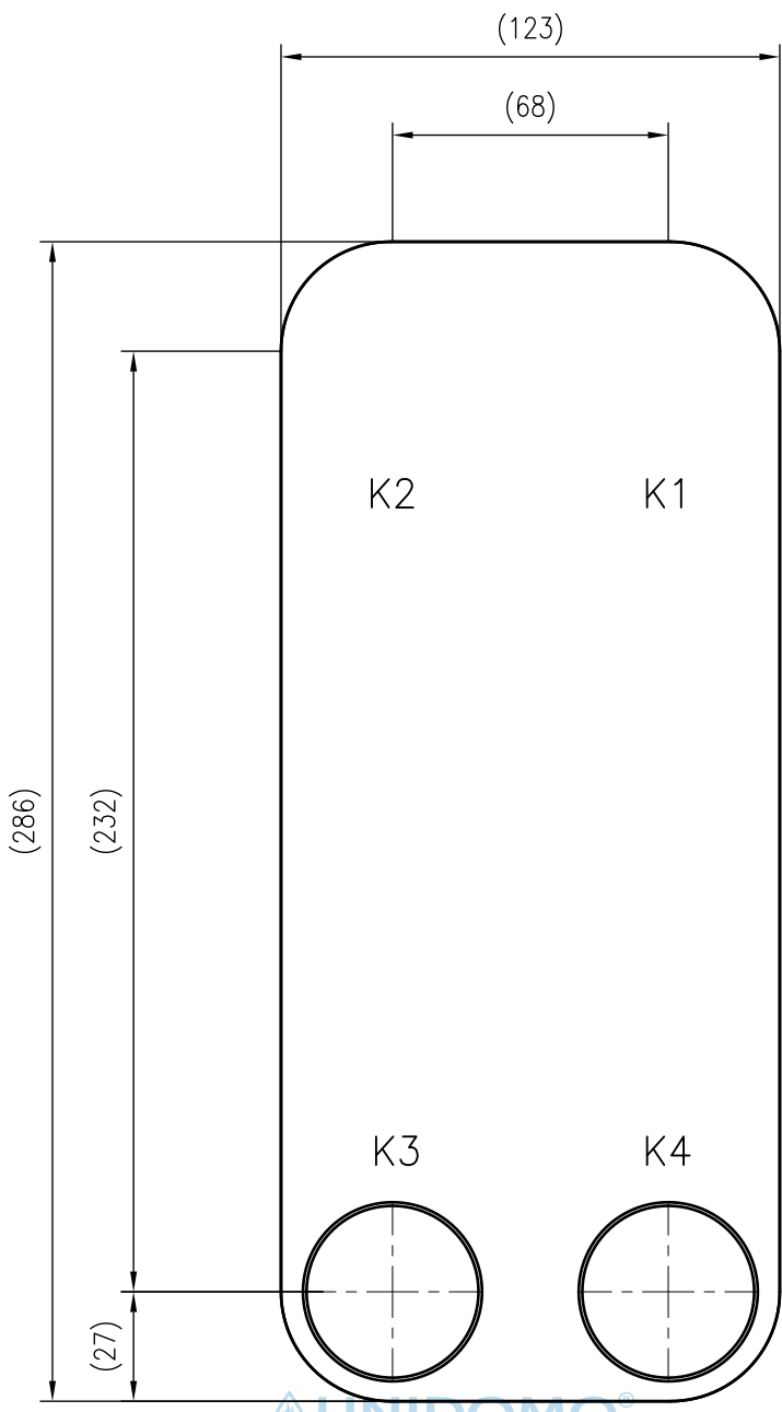
Front view
