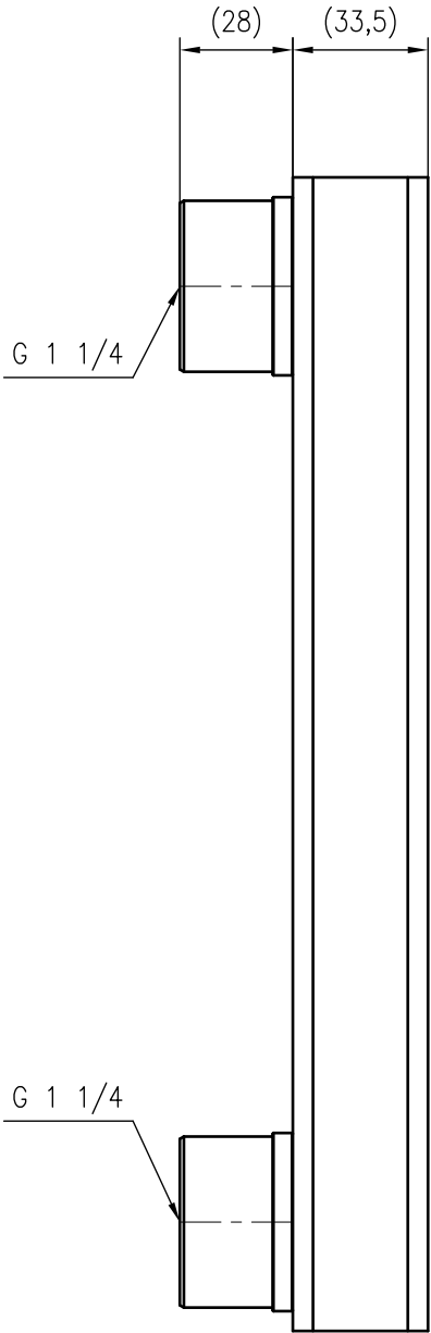
Side view
