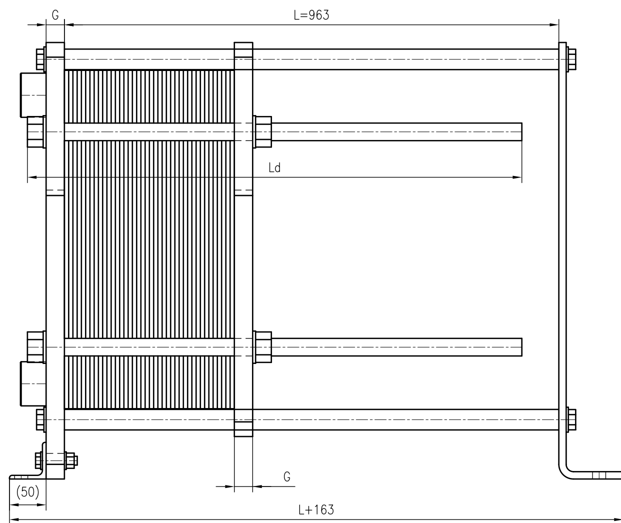
Side view
