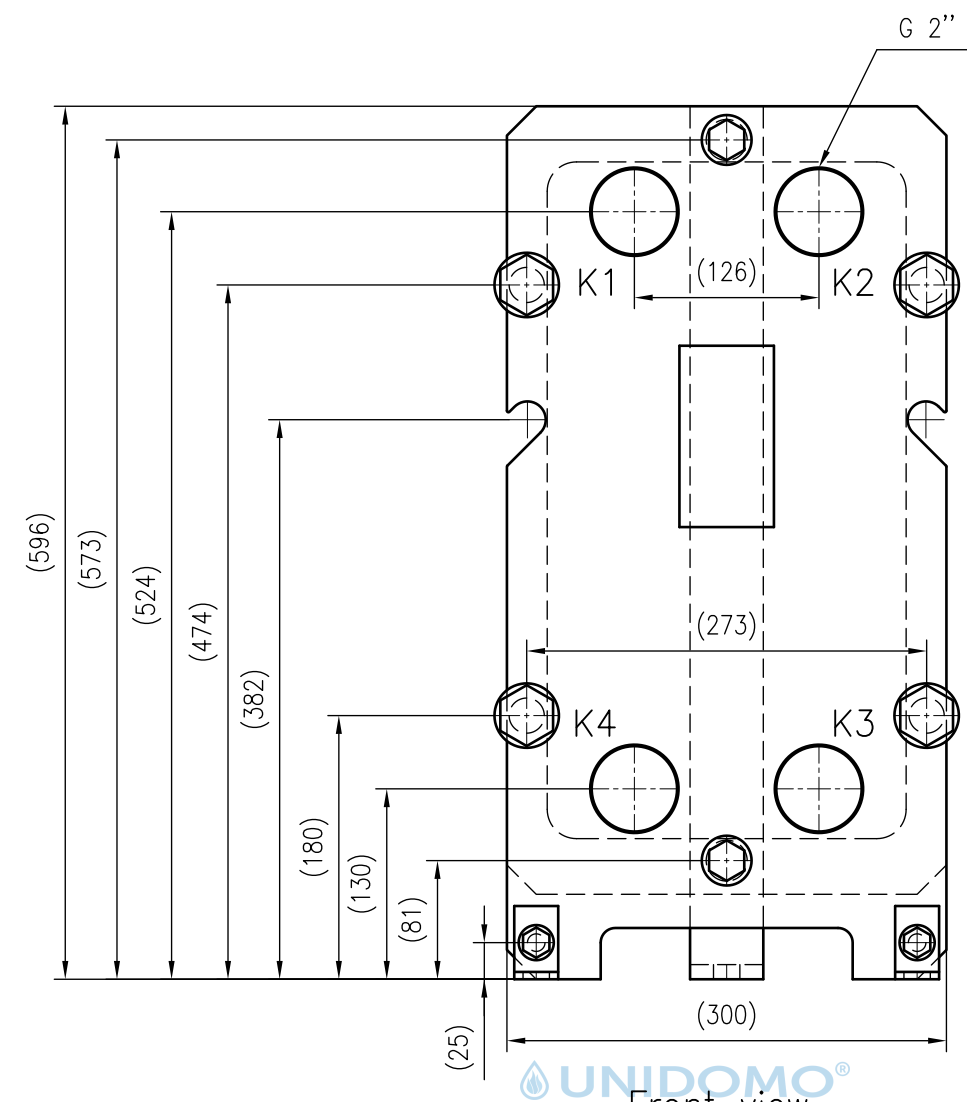
Front view
