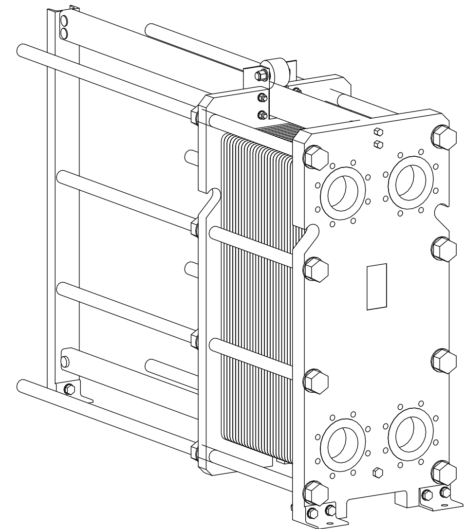
Isometric view
