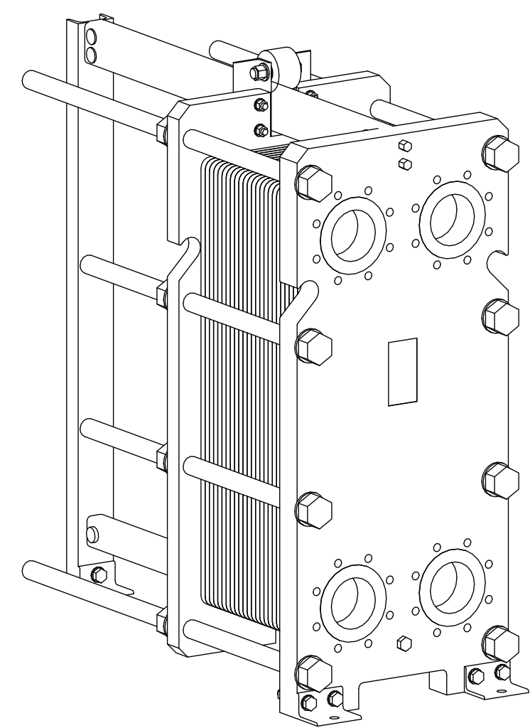
Isometric view
