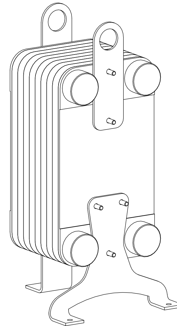
Isometric view
