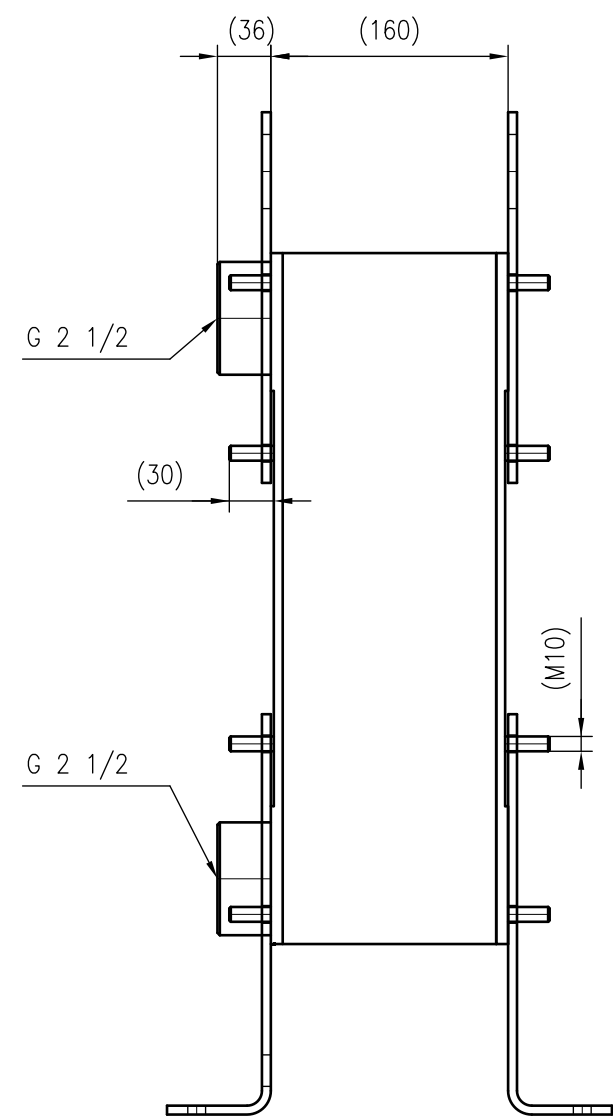
Side view
