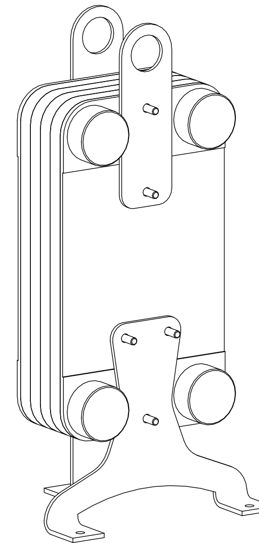
Isometric view
