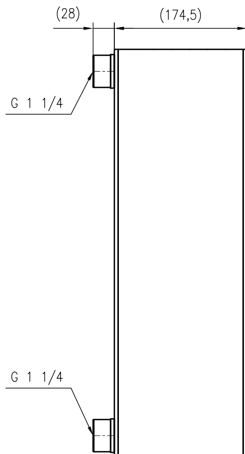
Side view
