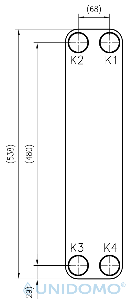
Front view
