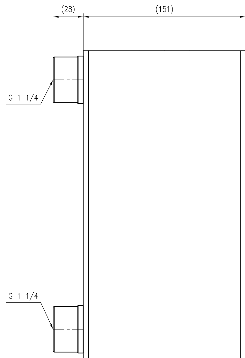
Side view
