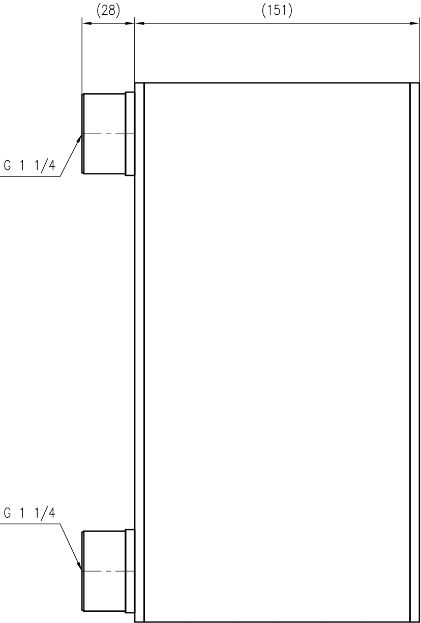
Side view
