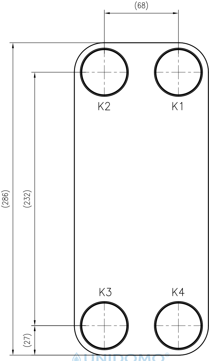
Front view
