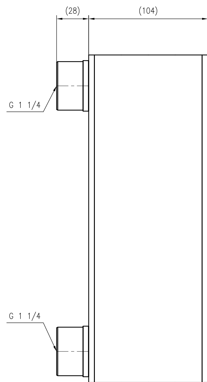
Side view
