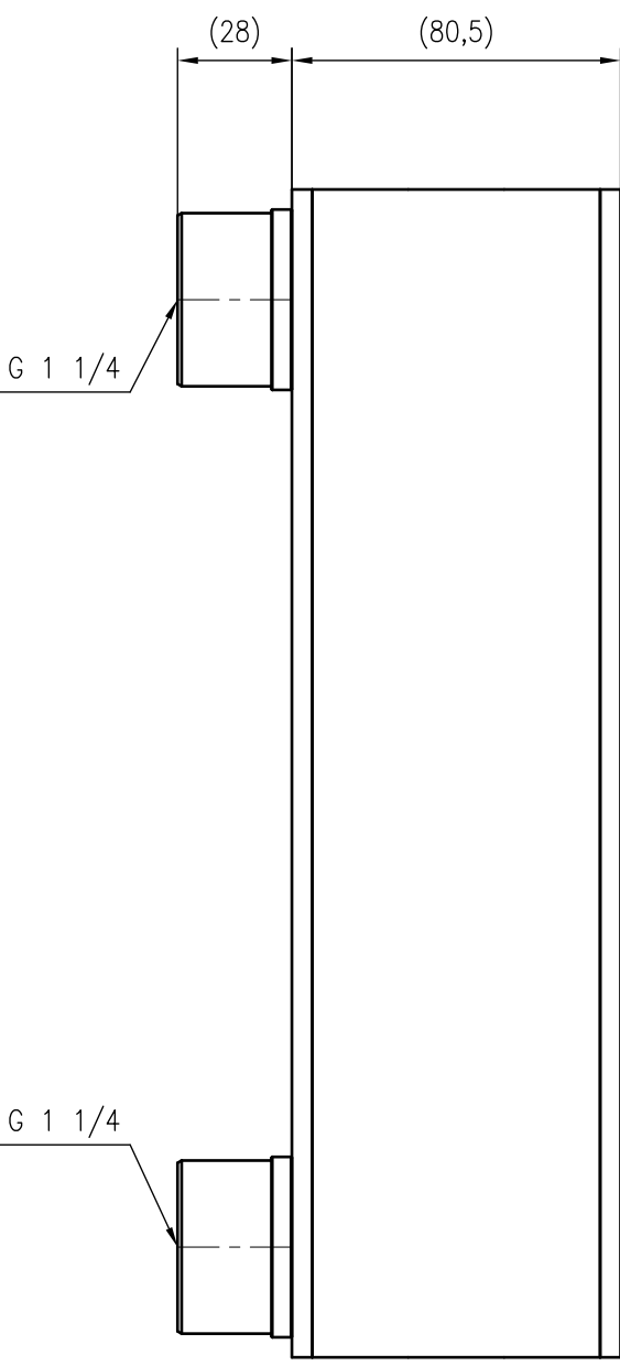
Side view
