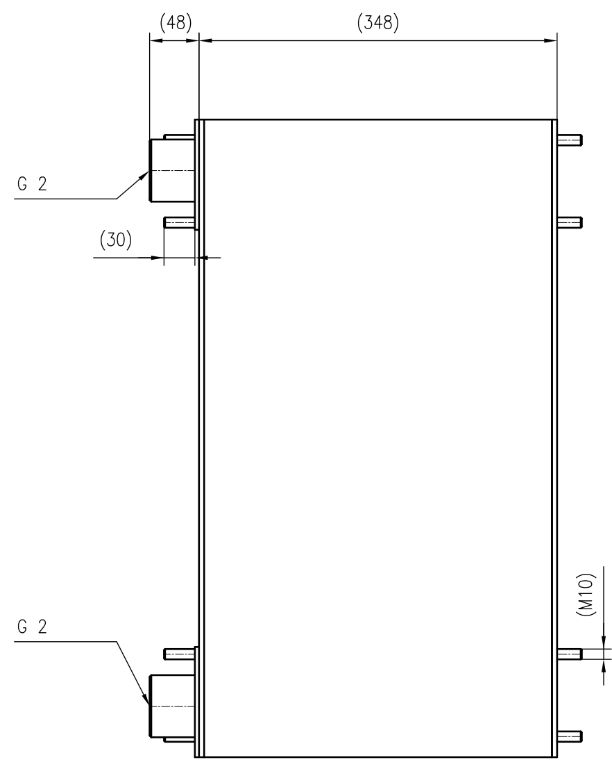
Side view
