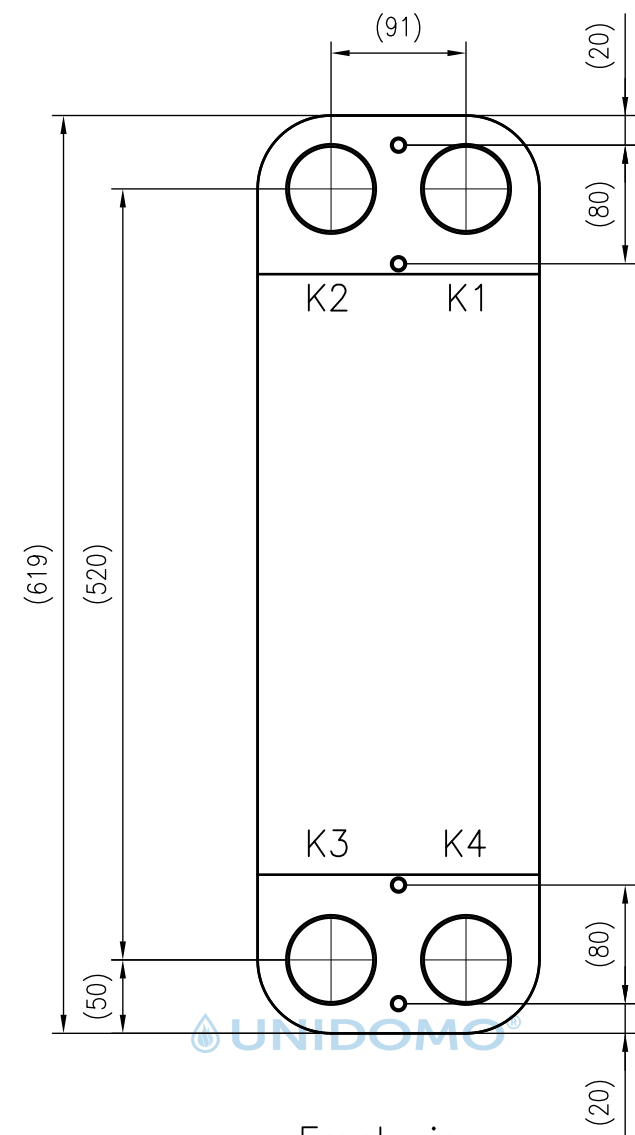
Front view
