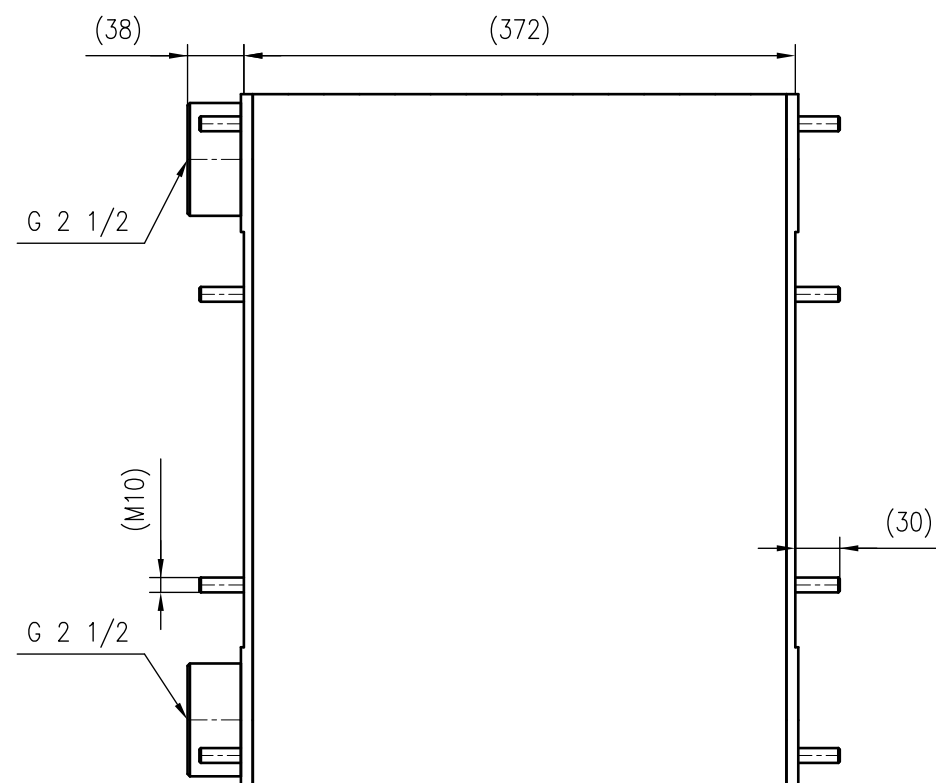
Side view
