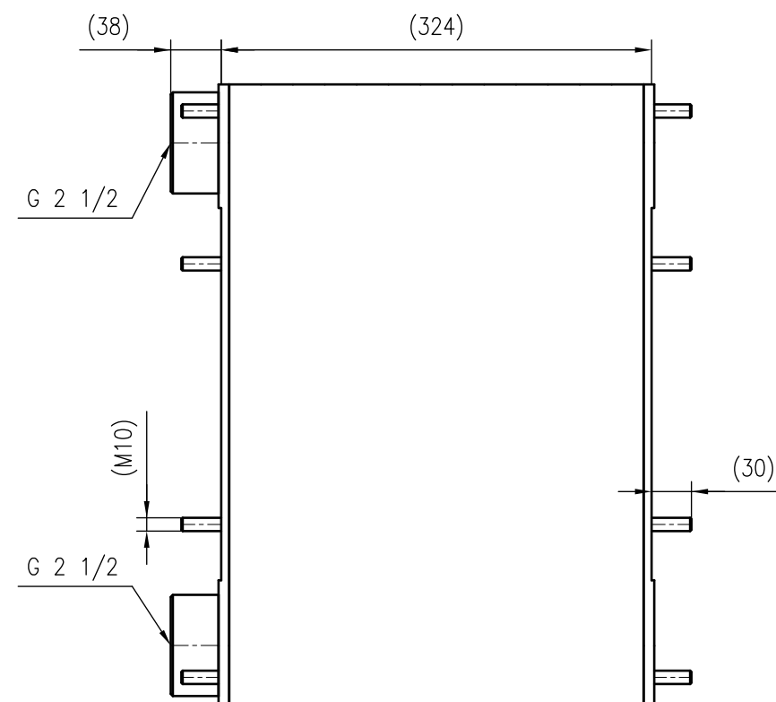
Side view
