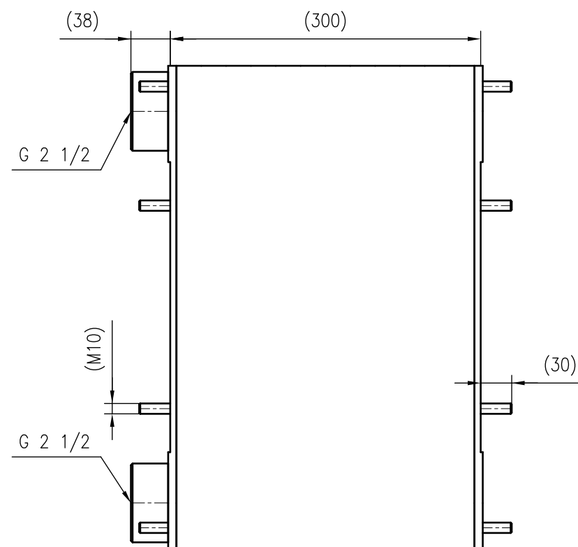
Side view
