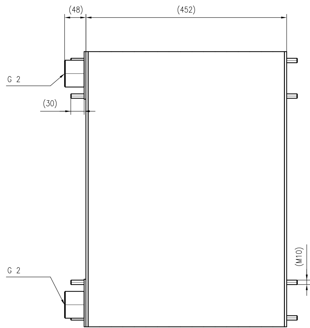
Side view
