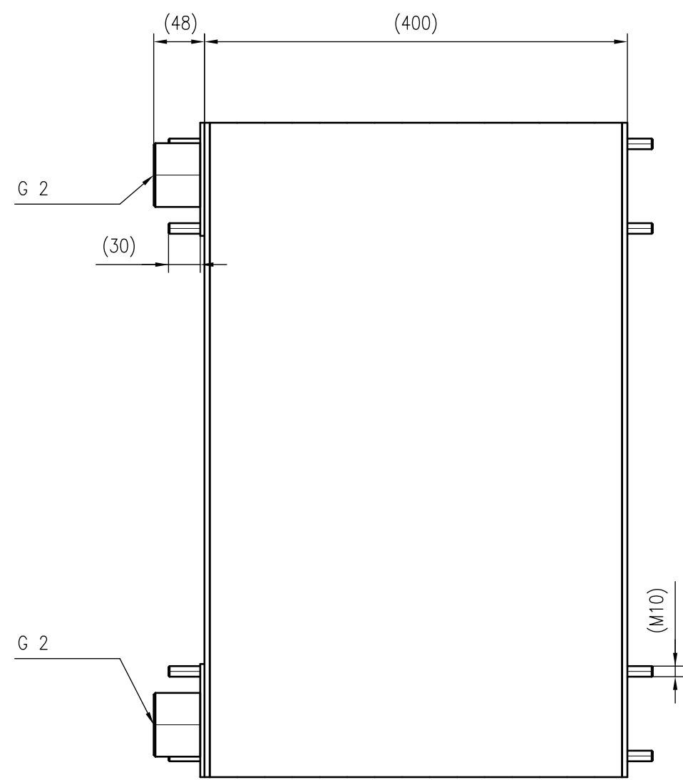
Side view
