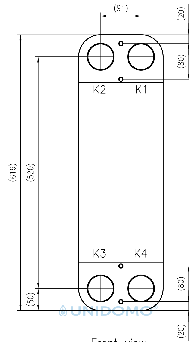
Front view
