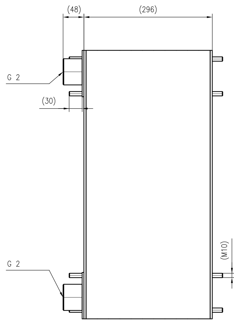
Side view
