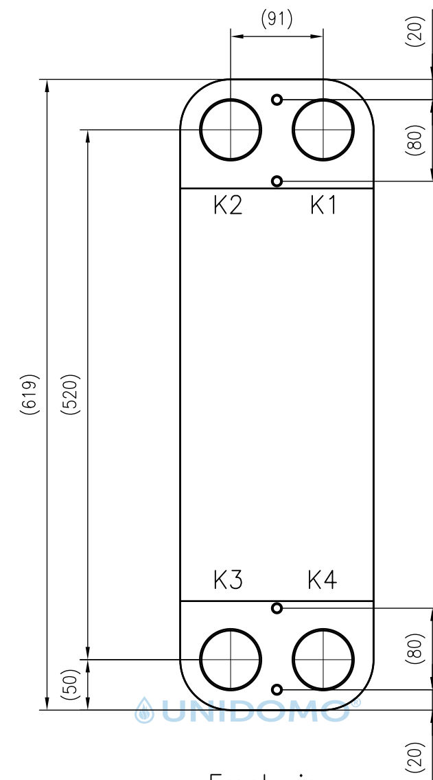
Front view
