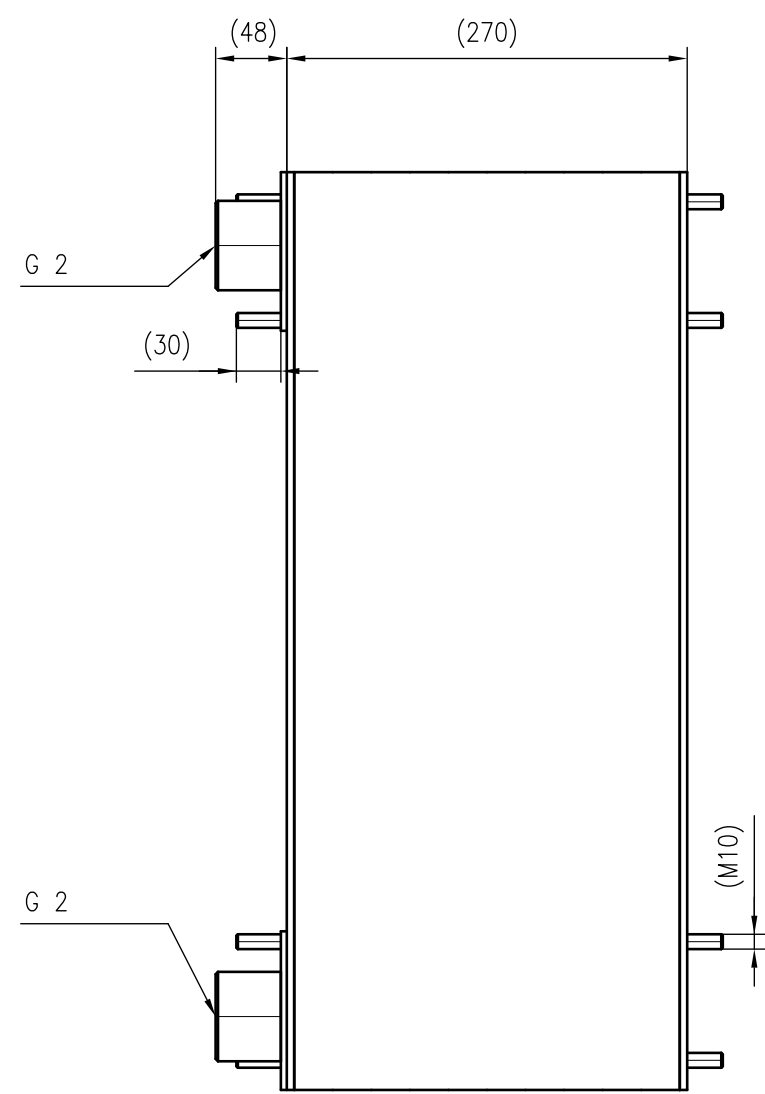
Side view
