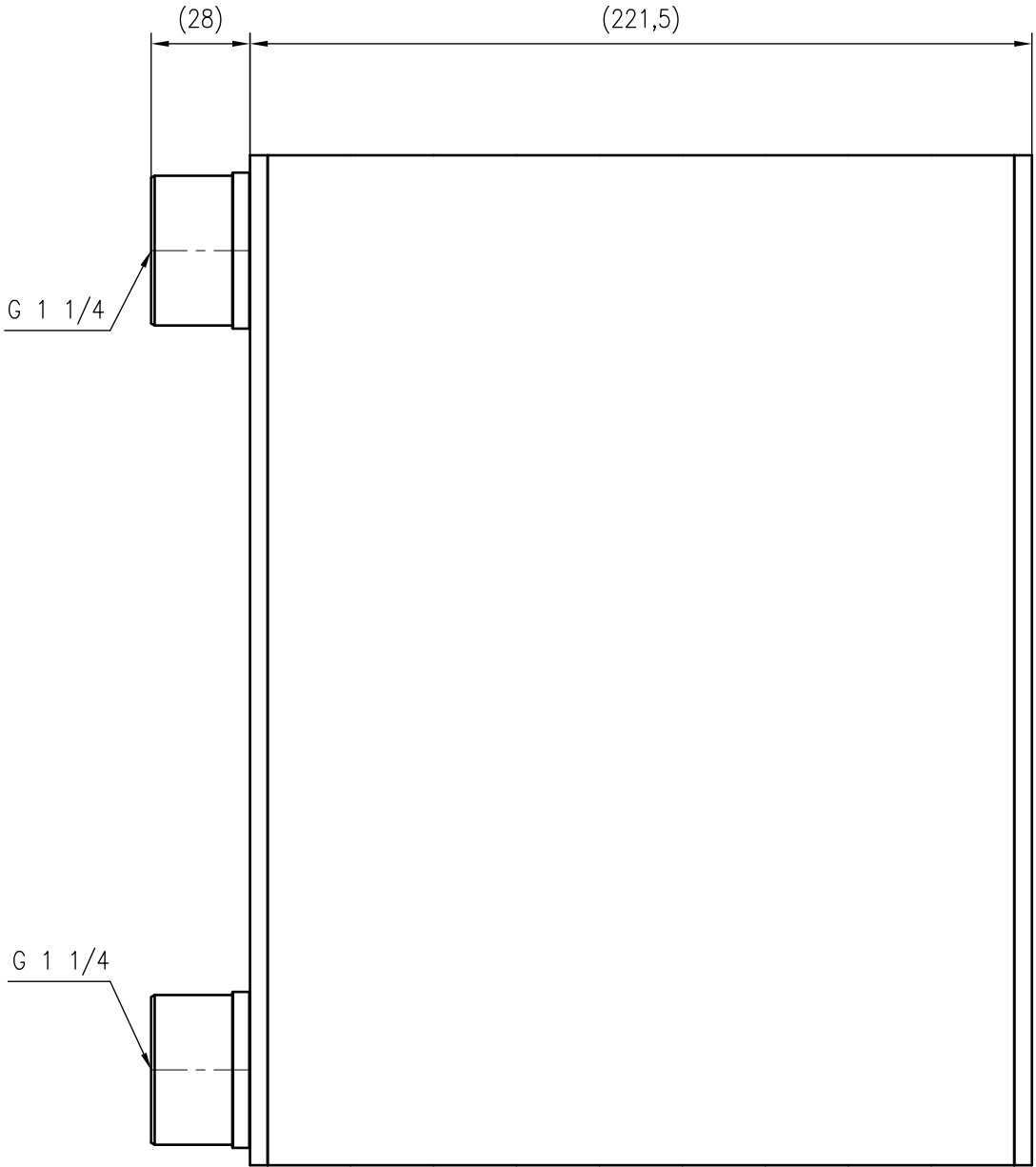
Side view
