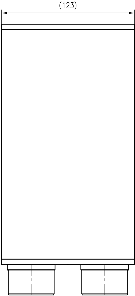
Top view
