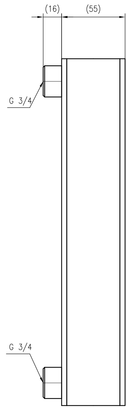
Side view
