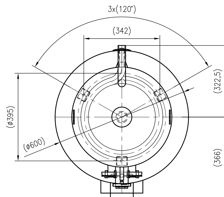
Top view
