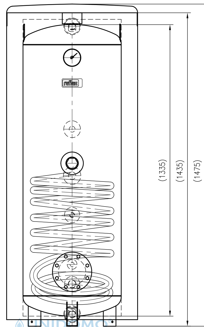
Front view
