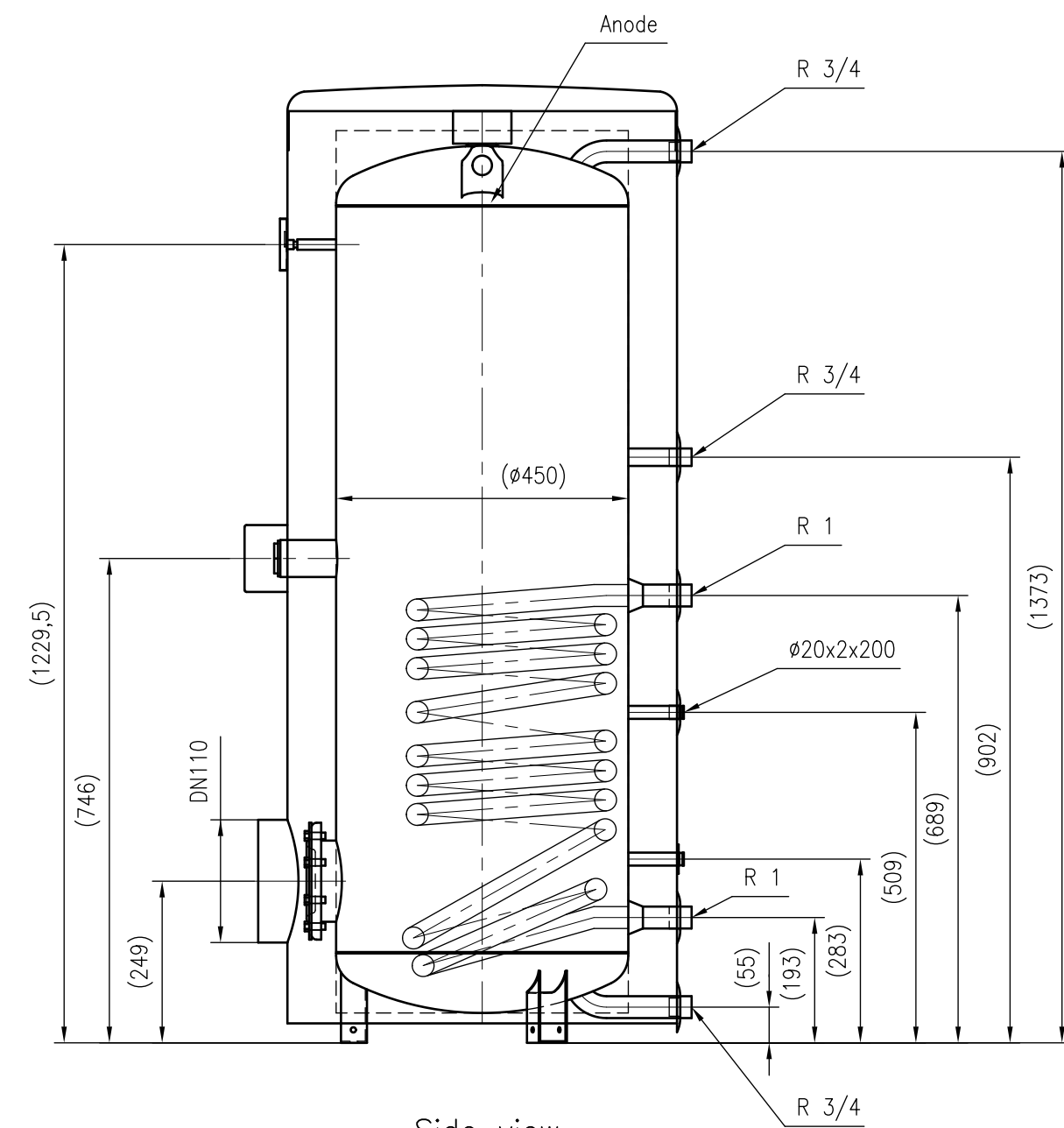
Side view
