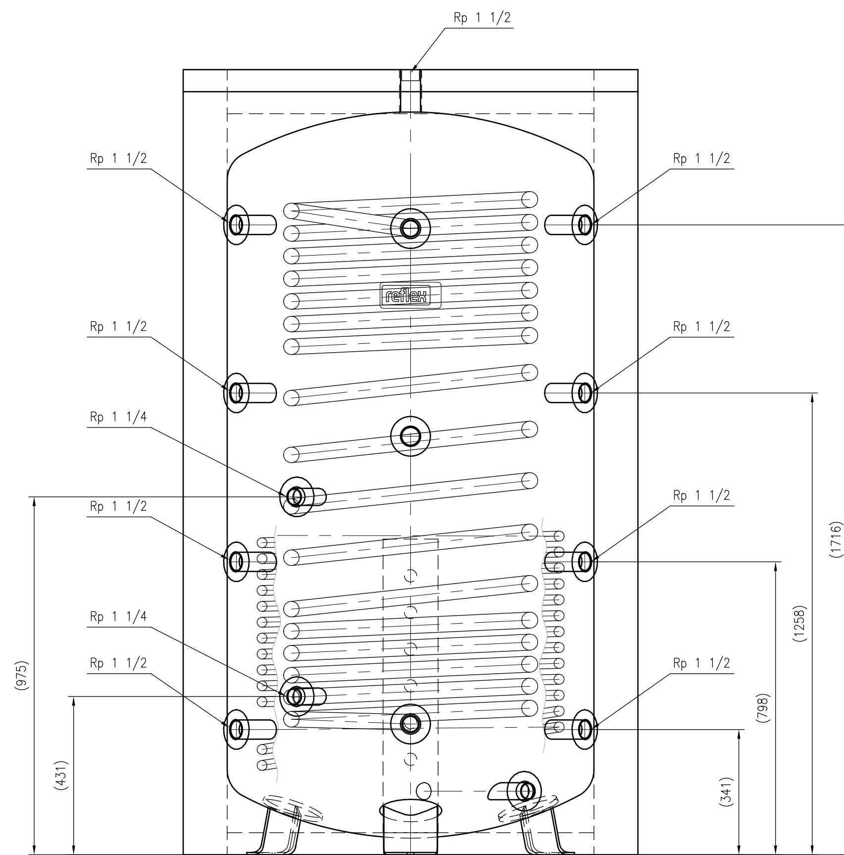
Front view
