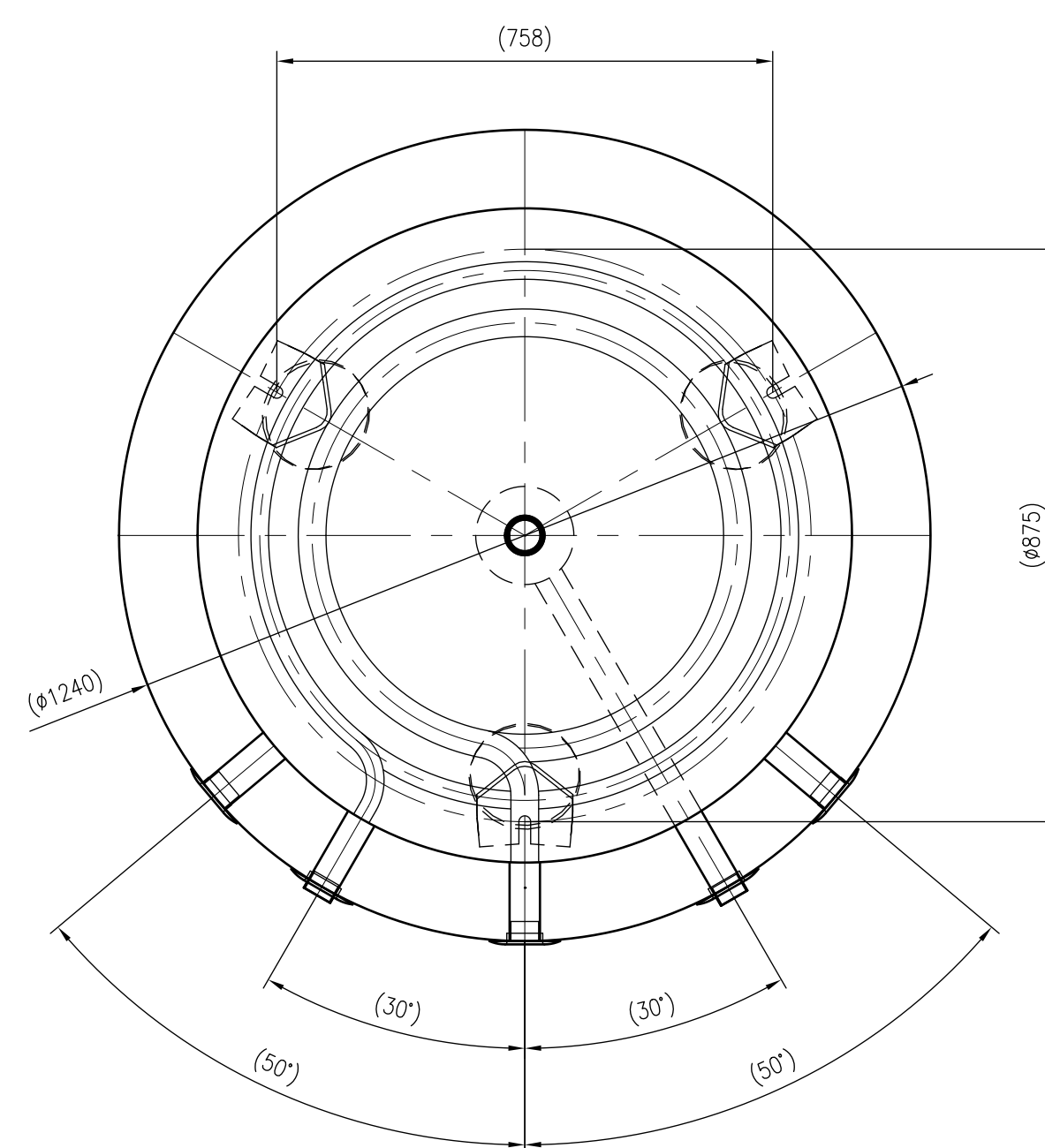
Top view
