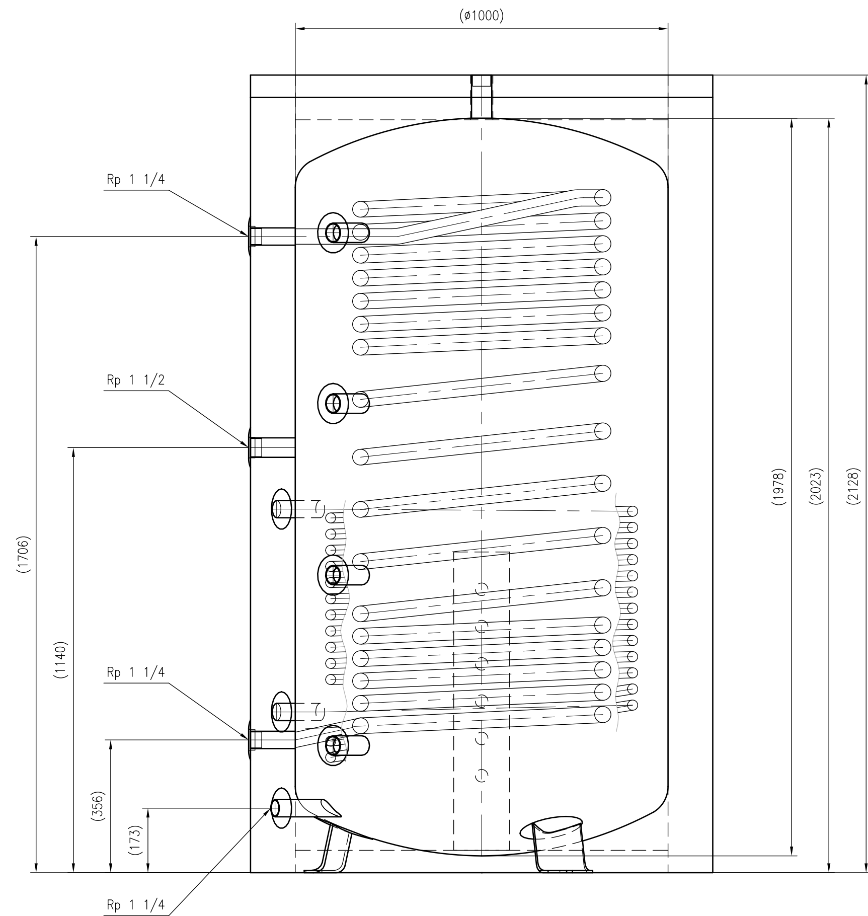
Side view
