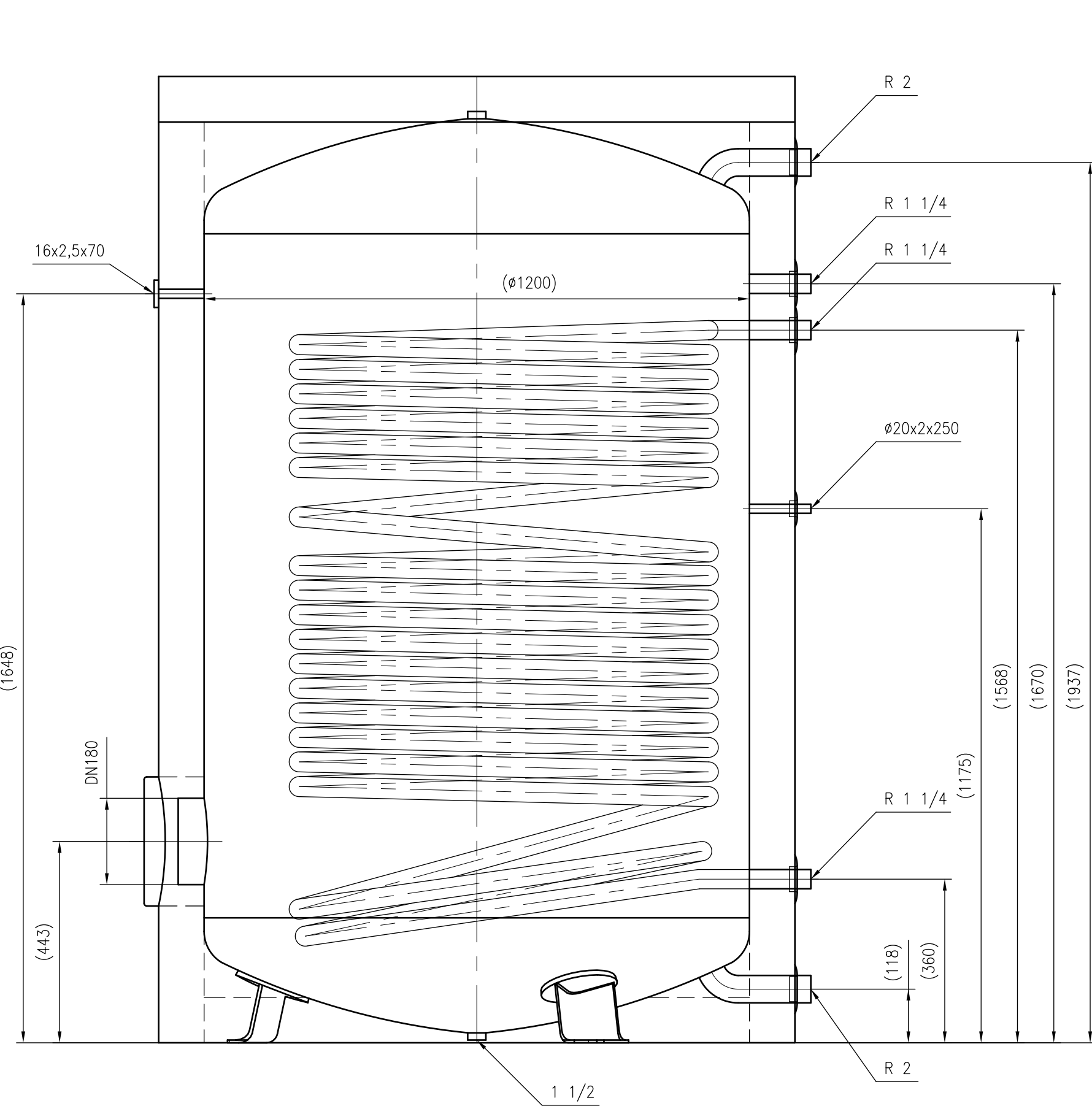
Side view
