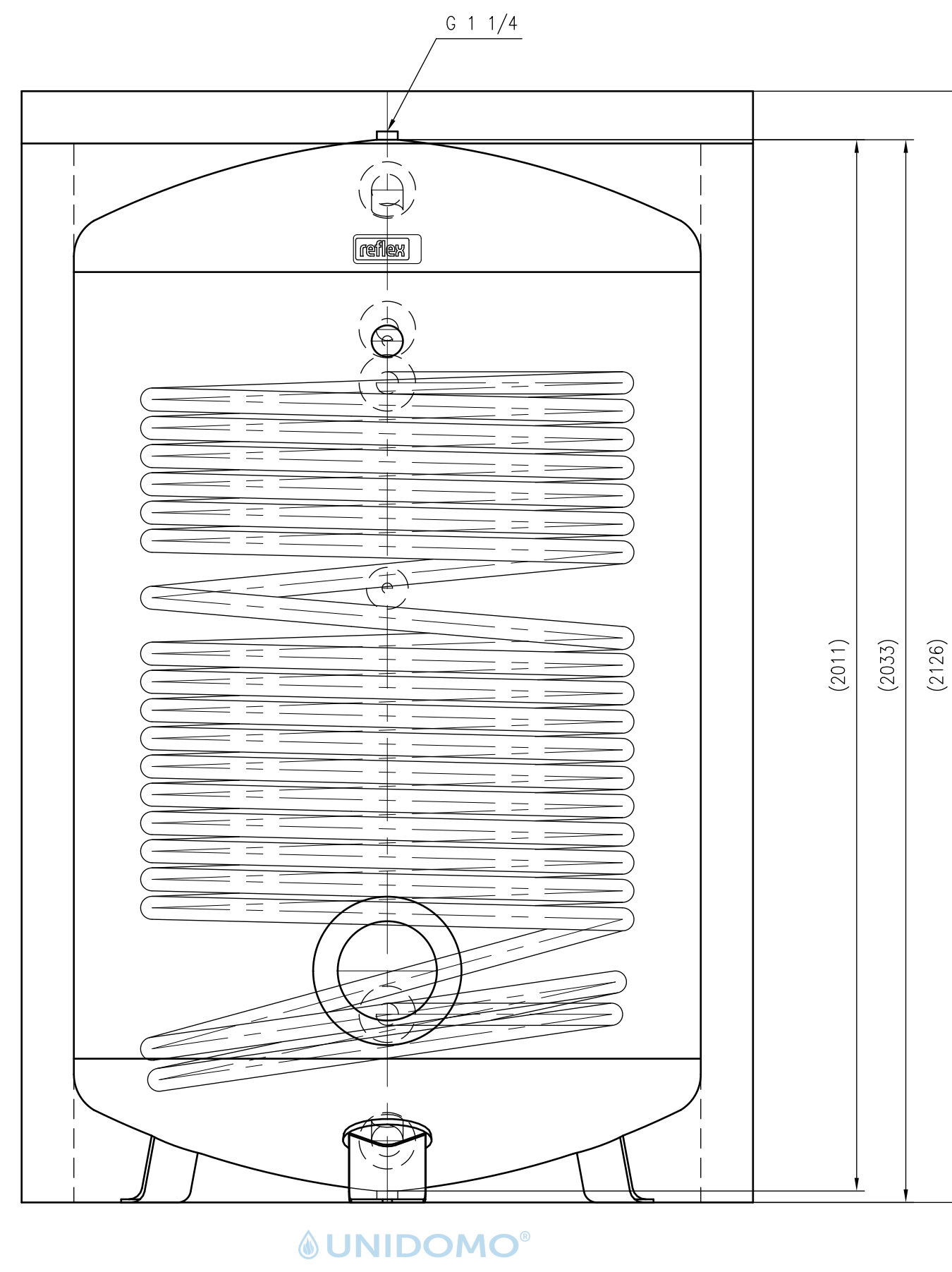
Front view
