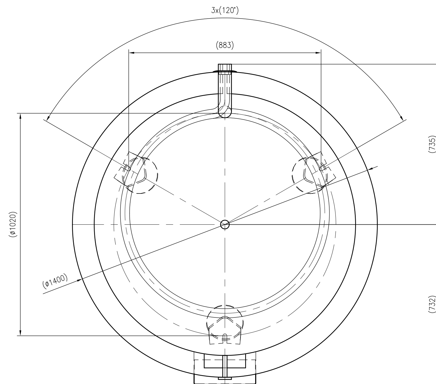
Top view
