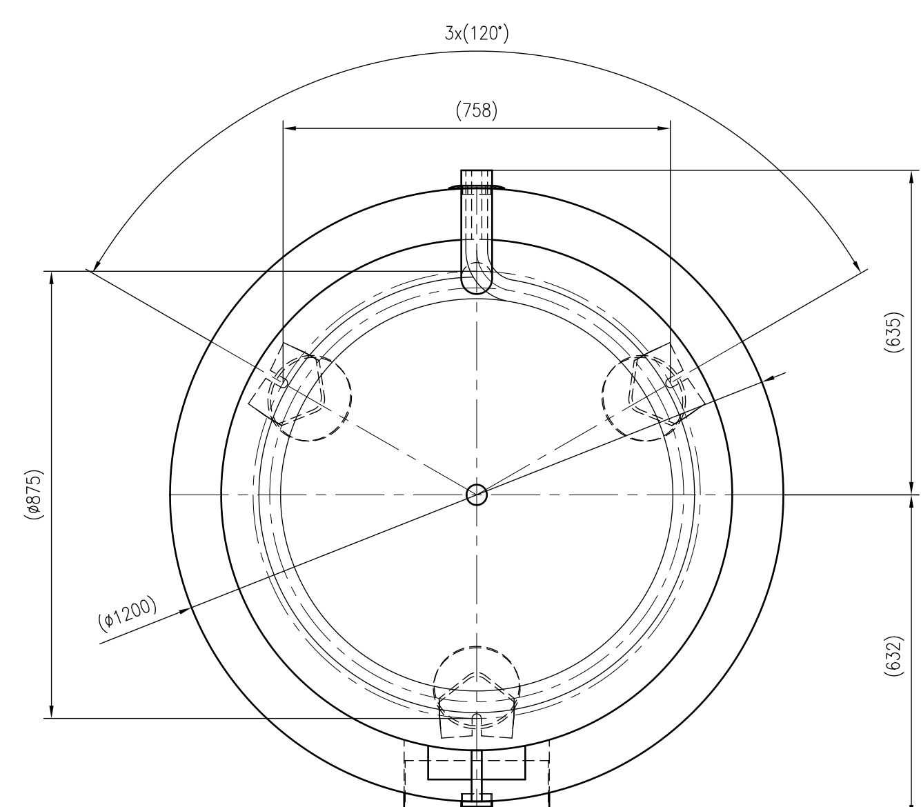
Top view
