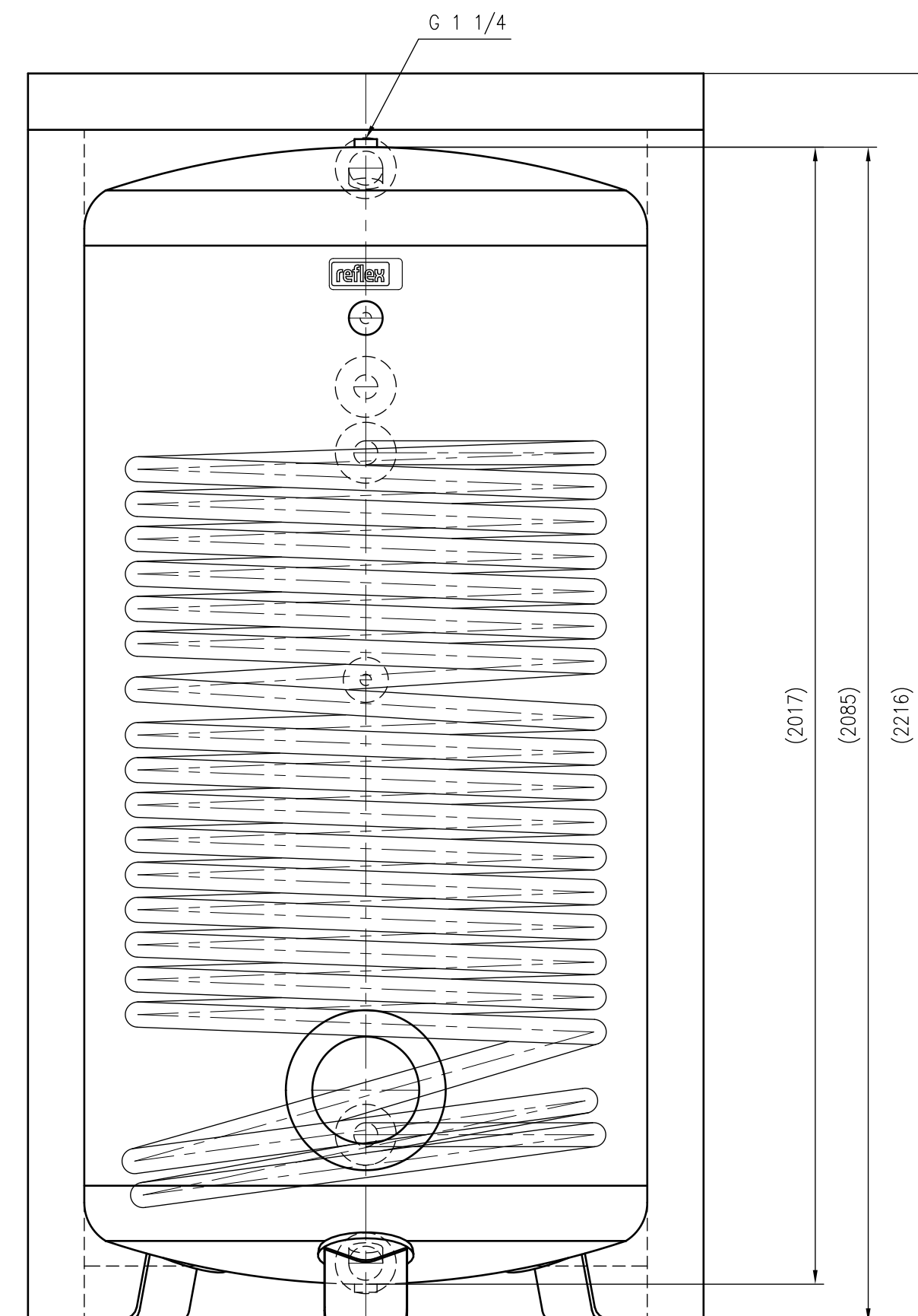
Front view
