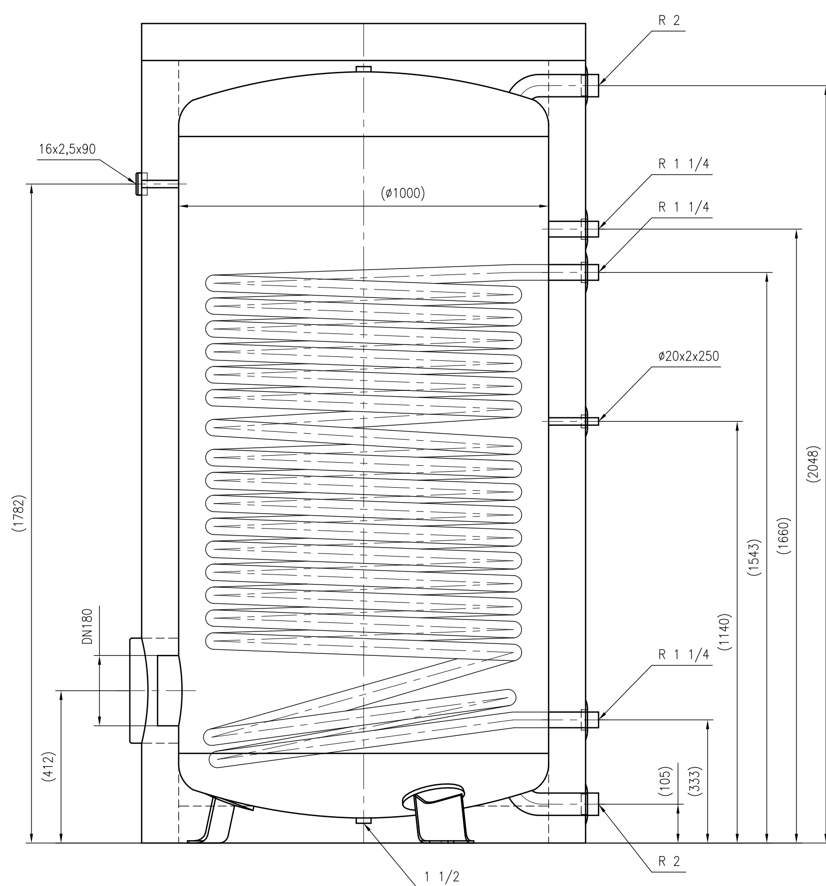
Side view
