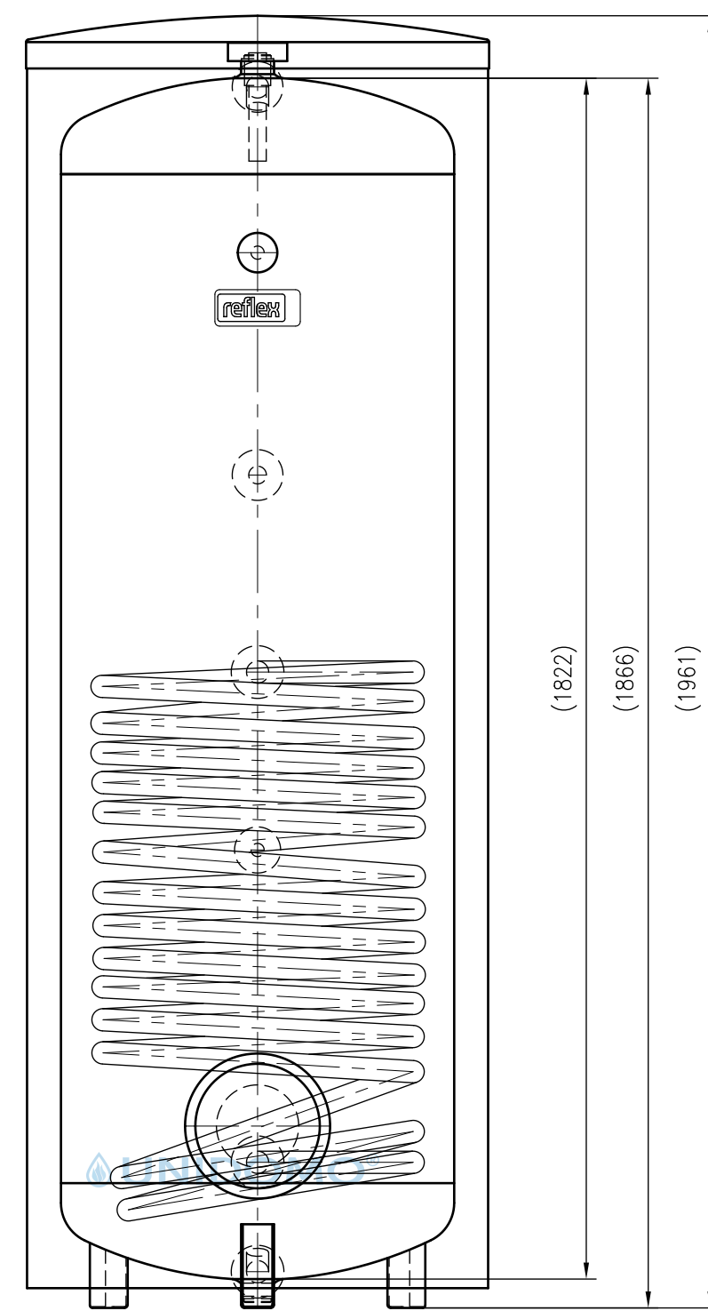
Front view
