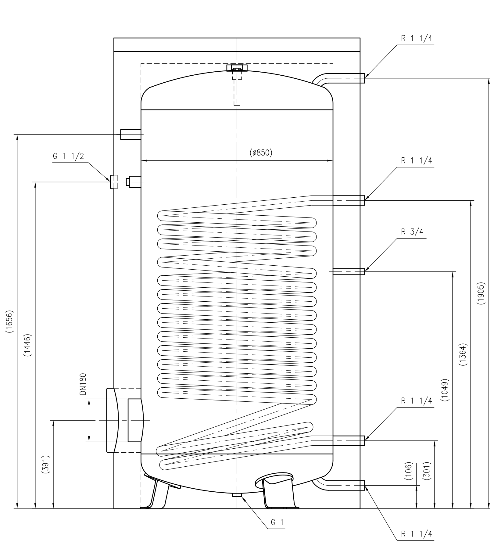
Side view
