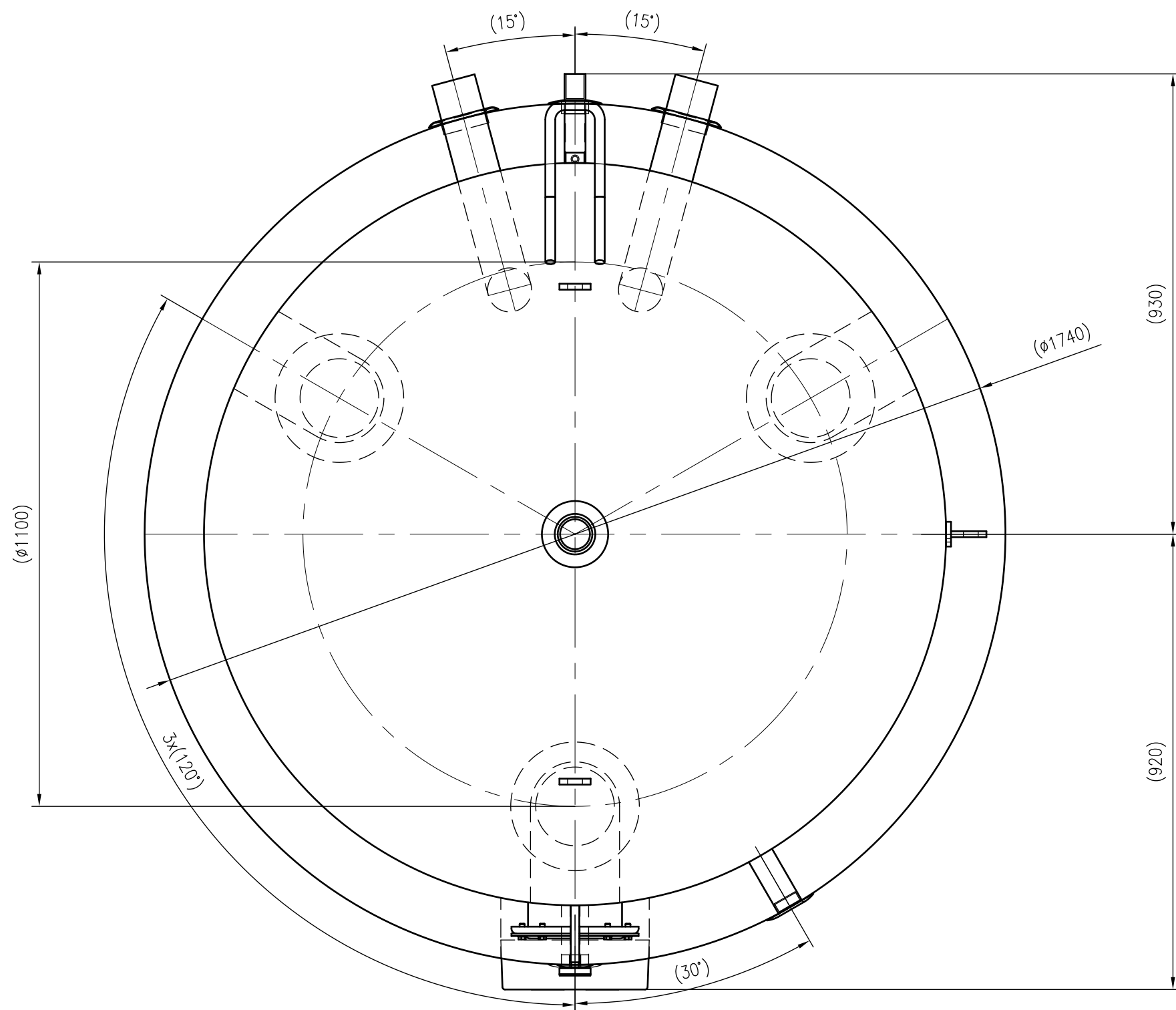
Top view
