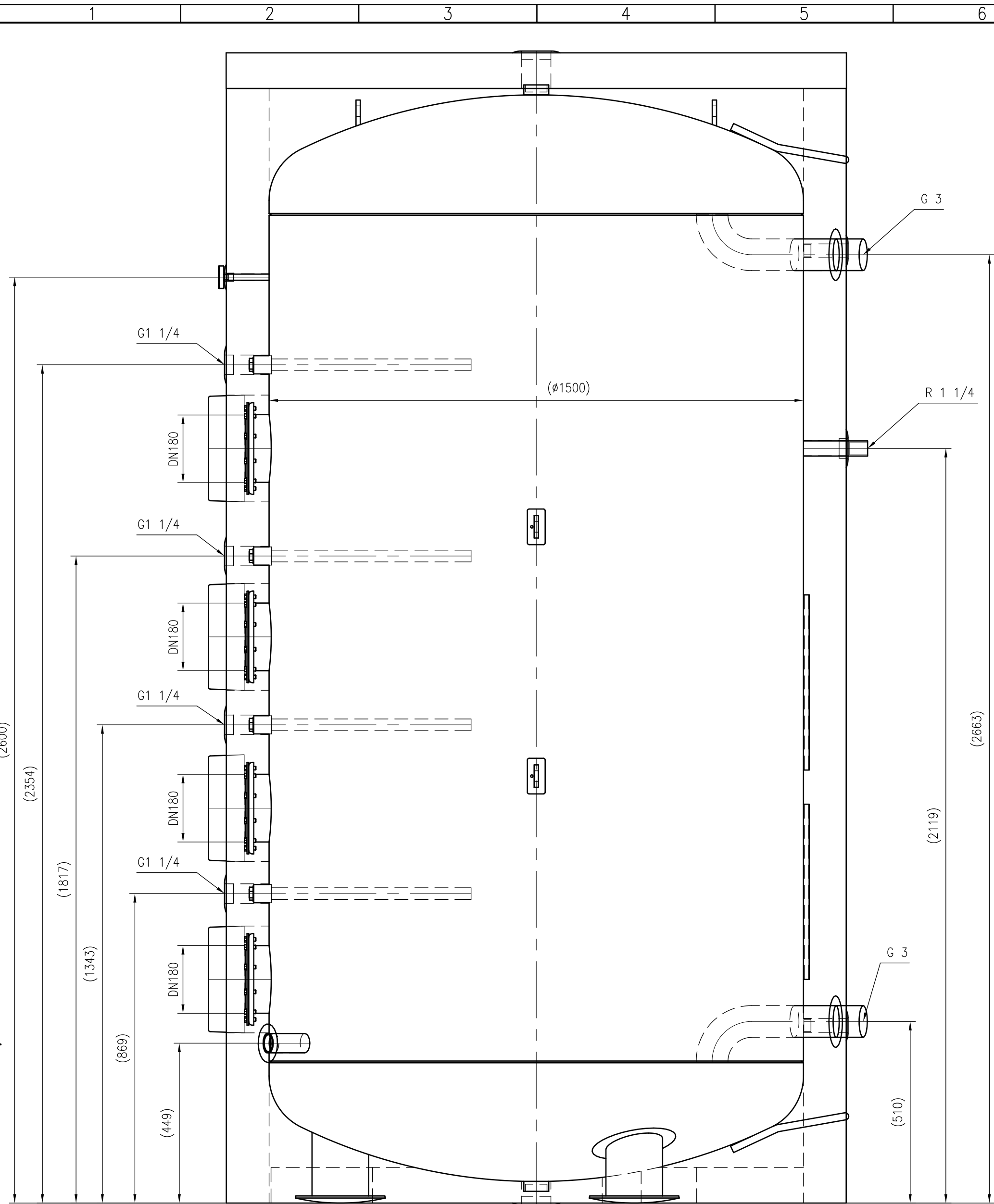
Side view
