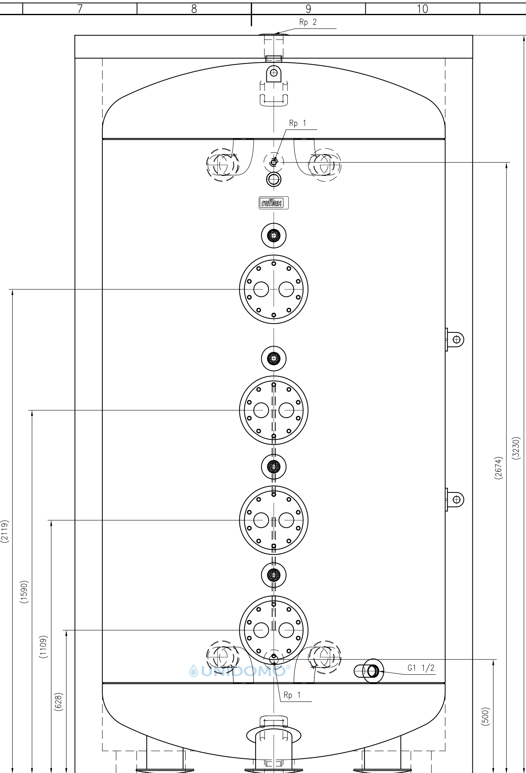
Front view
