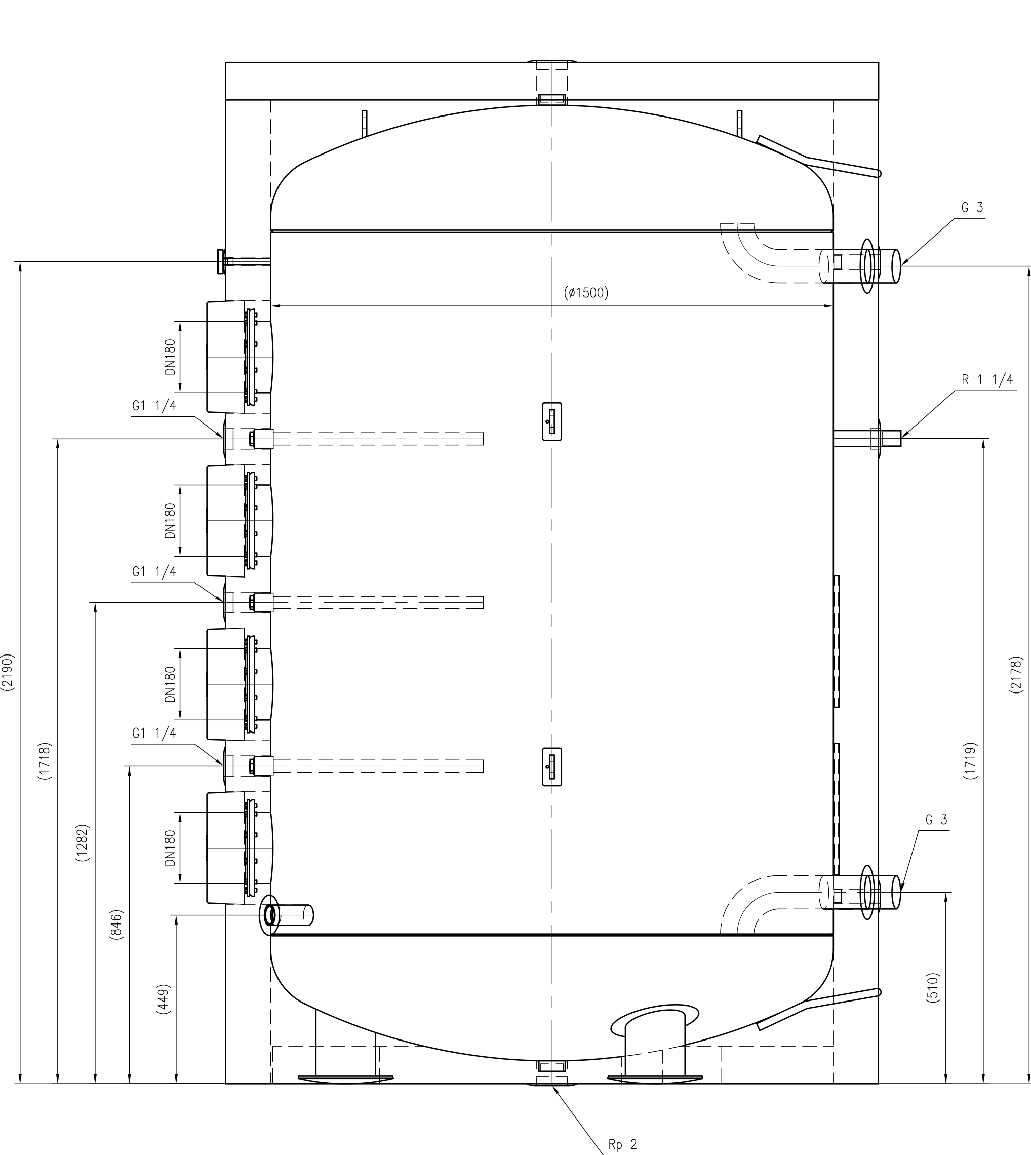
Side view
