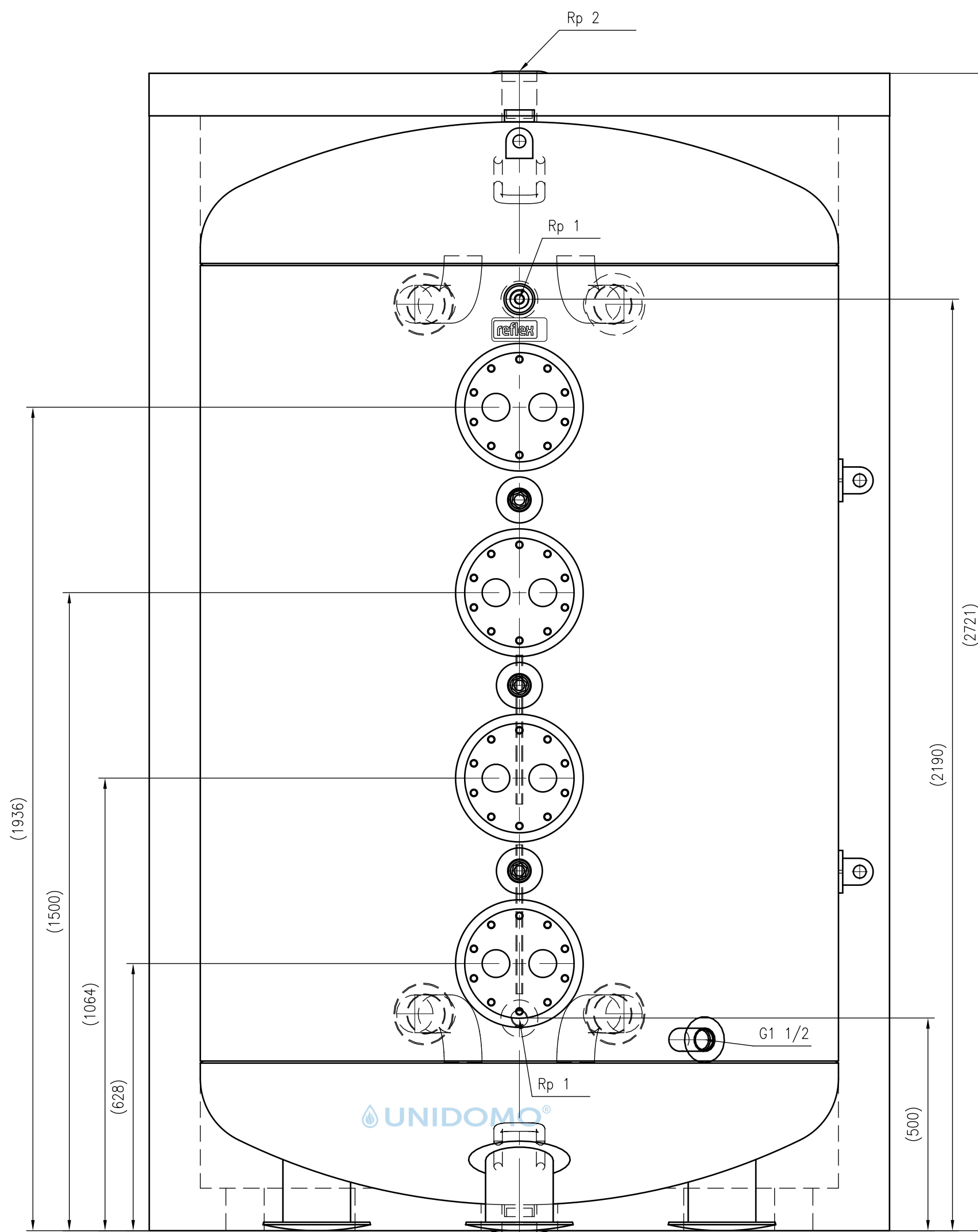
Front view
