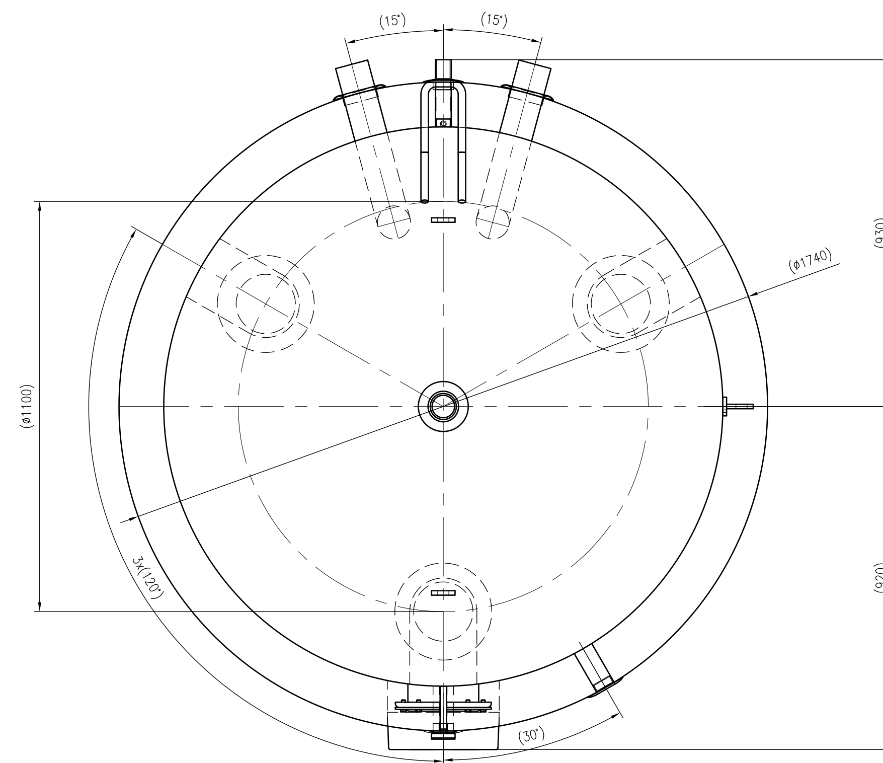
Top view
