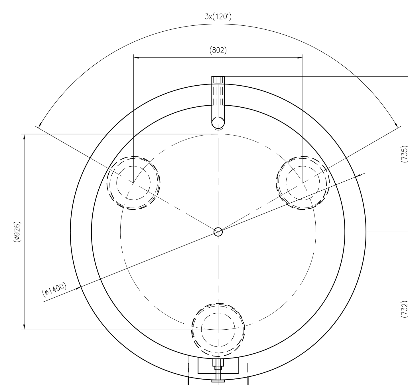
Top view
