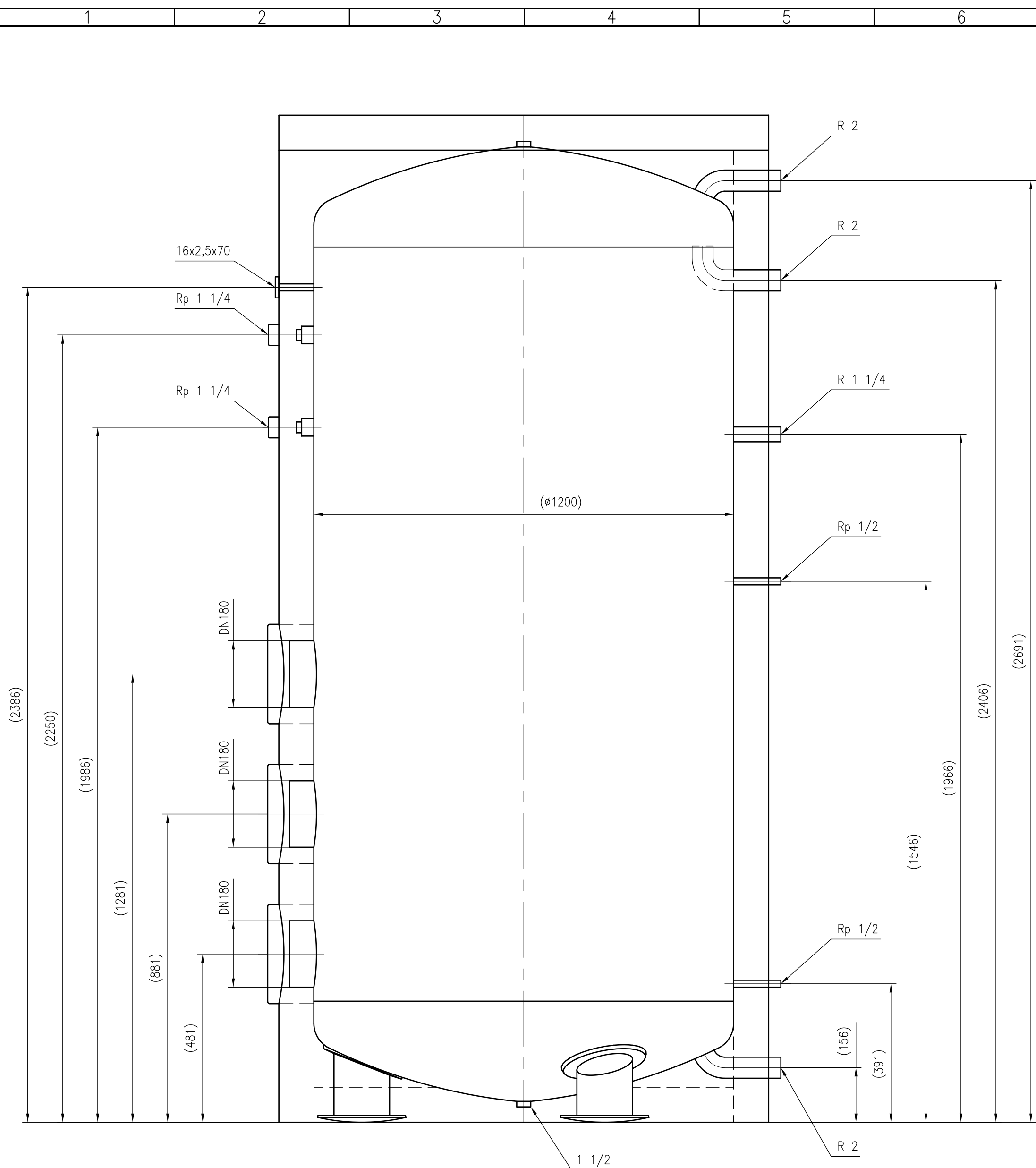
Side view
