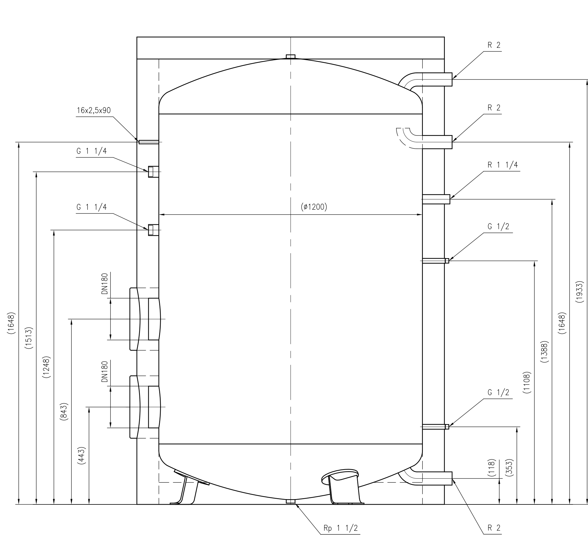
Side view
