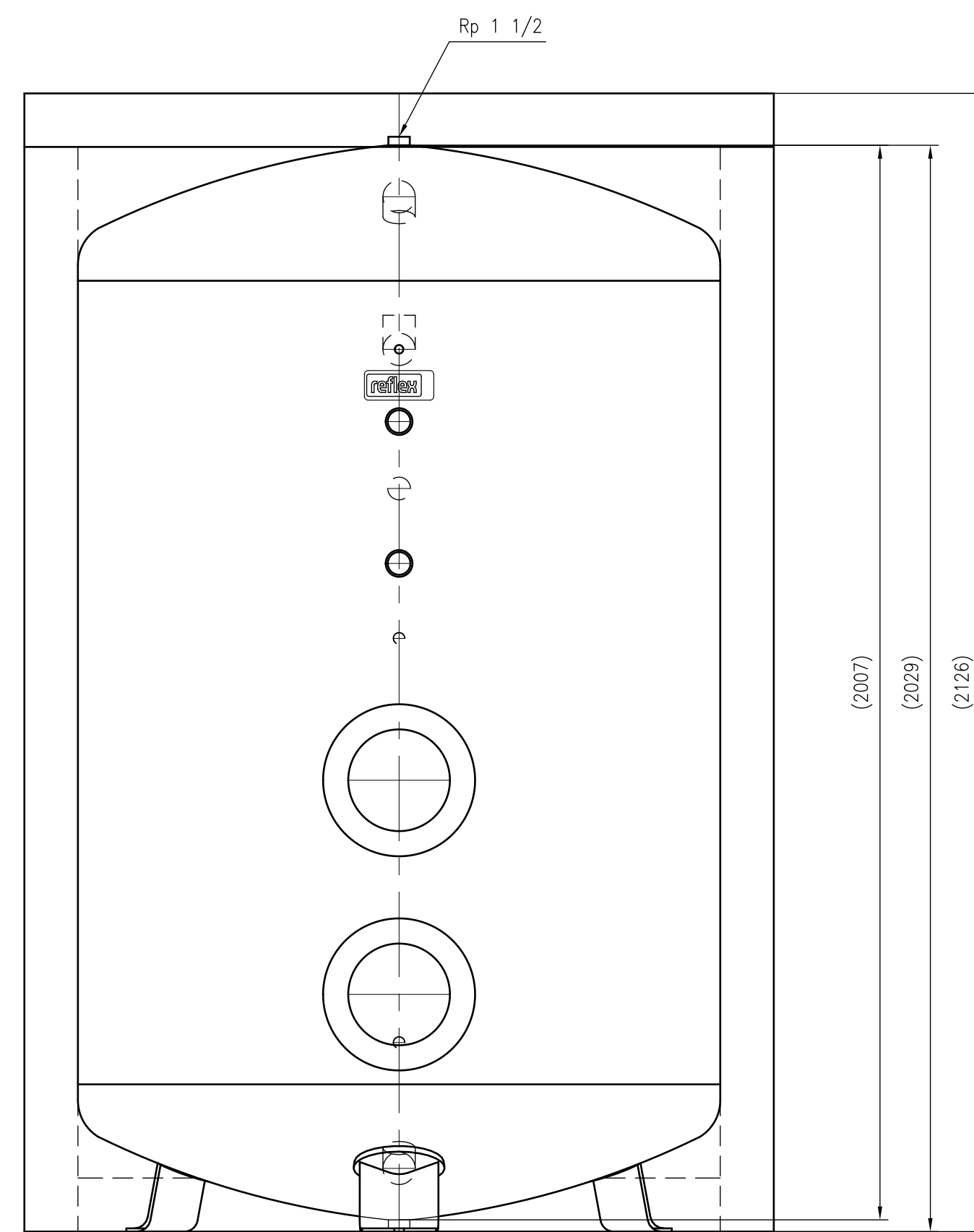
Front view
