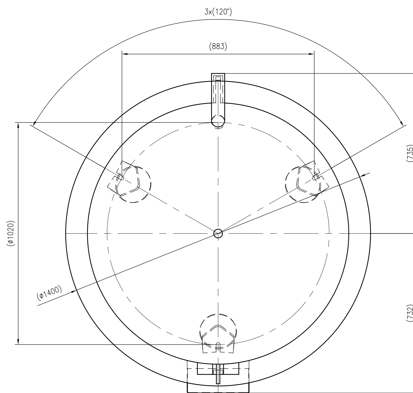
Top view
