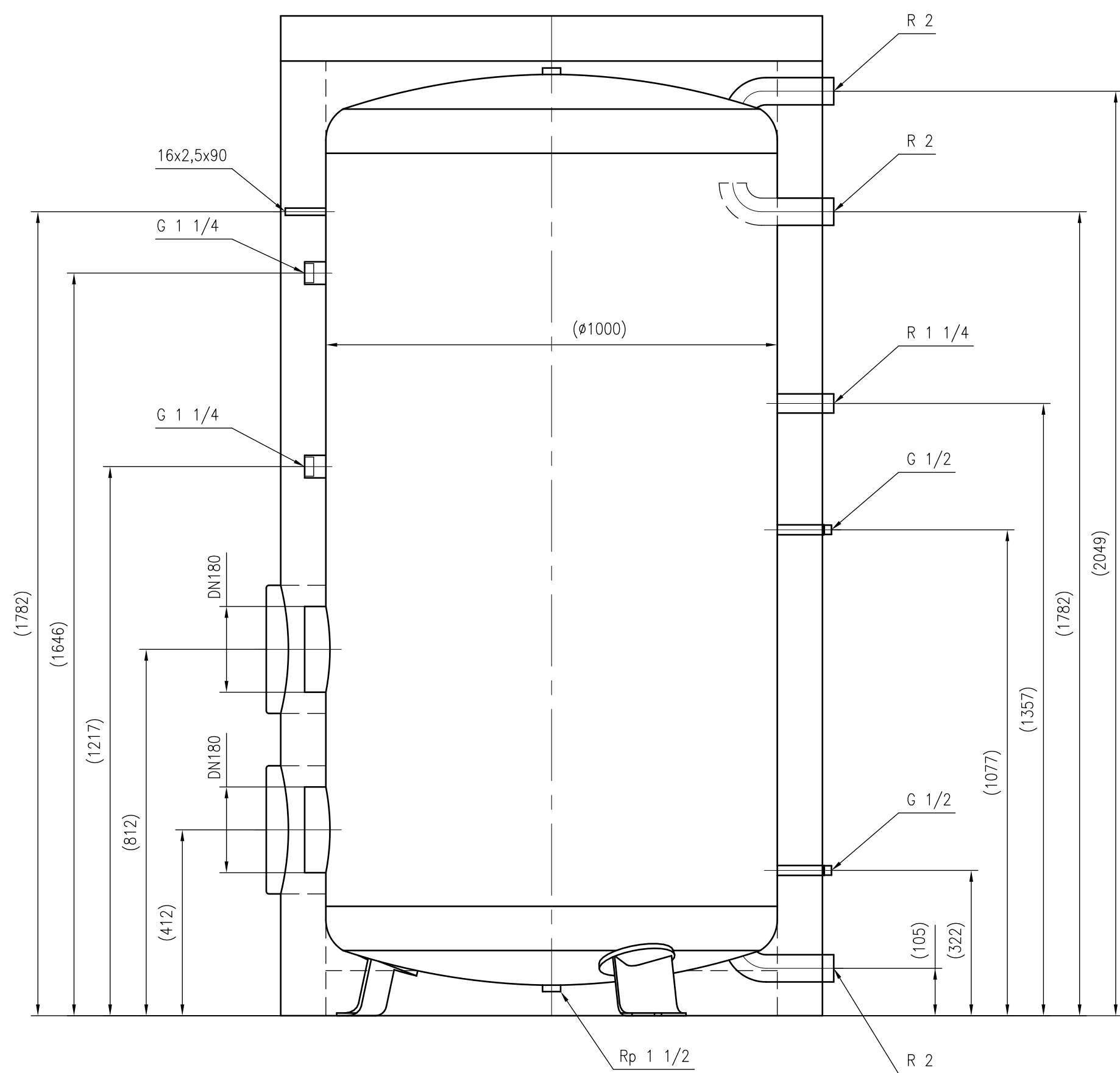
Side view
