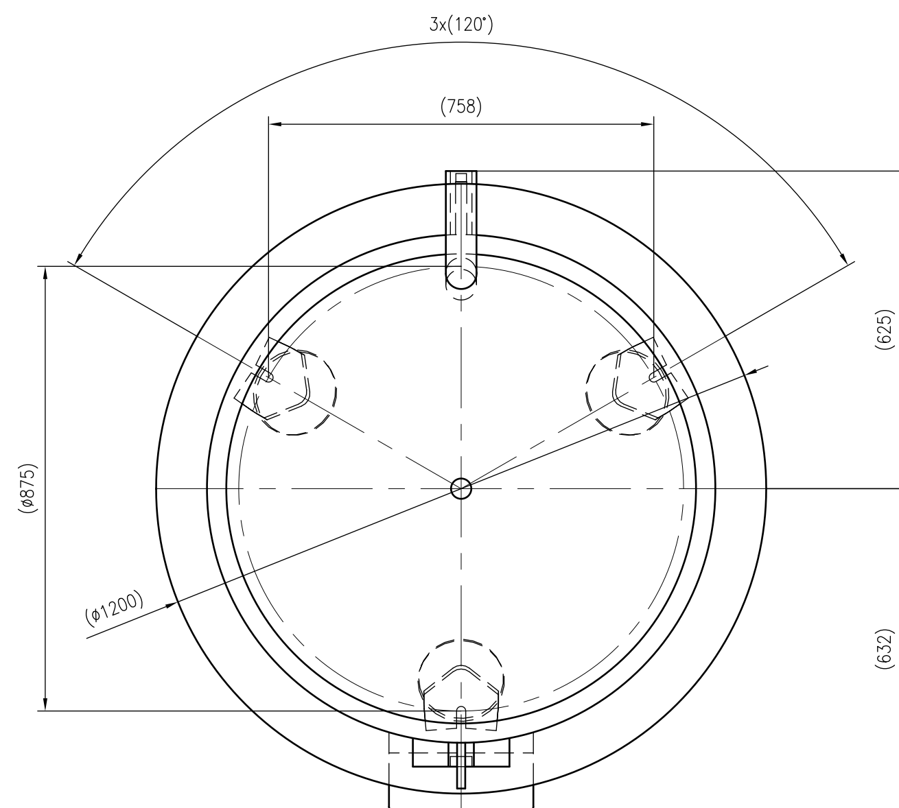
Top view
