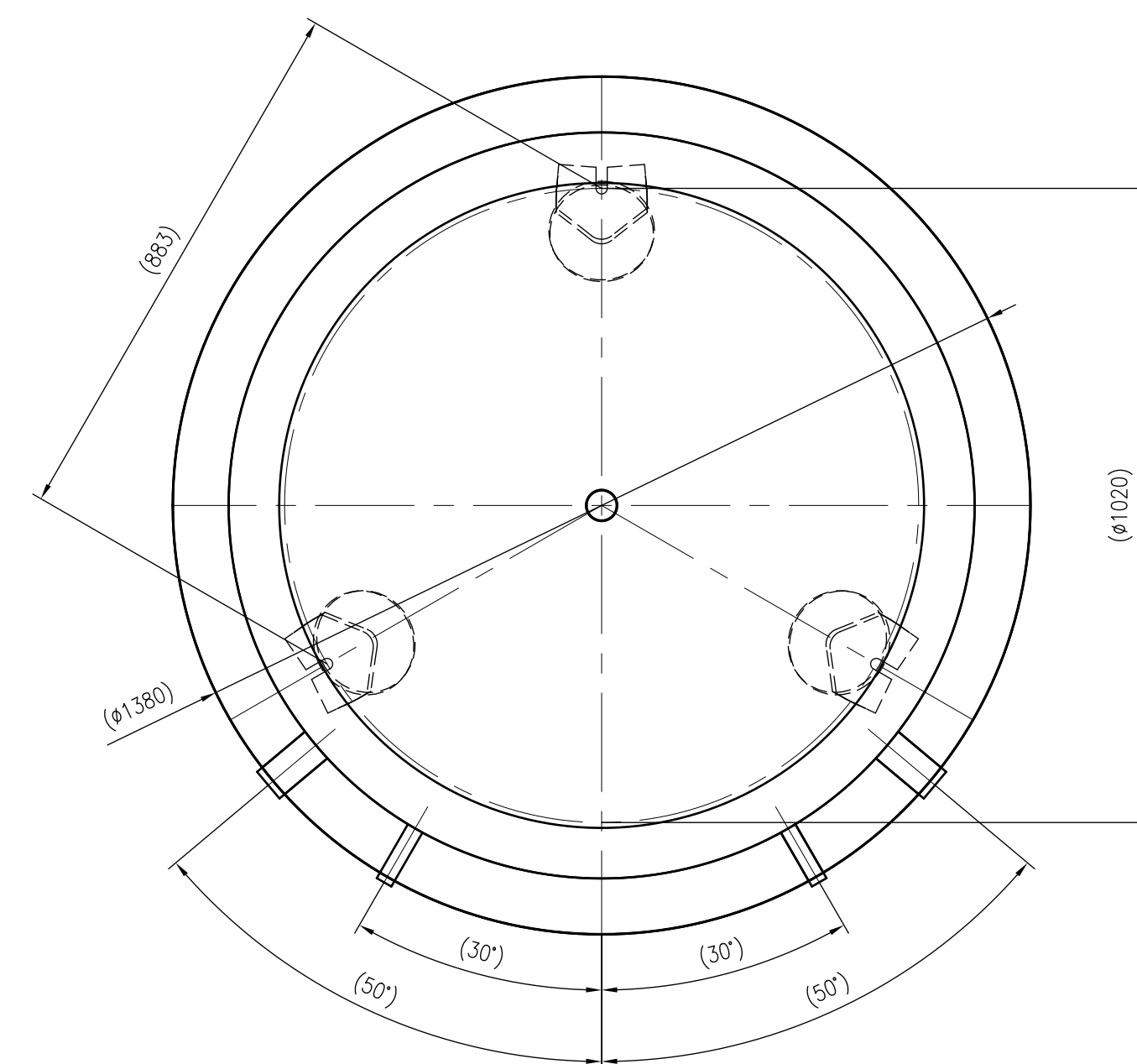
Top view
