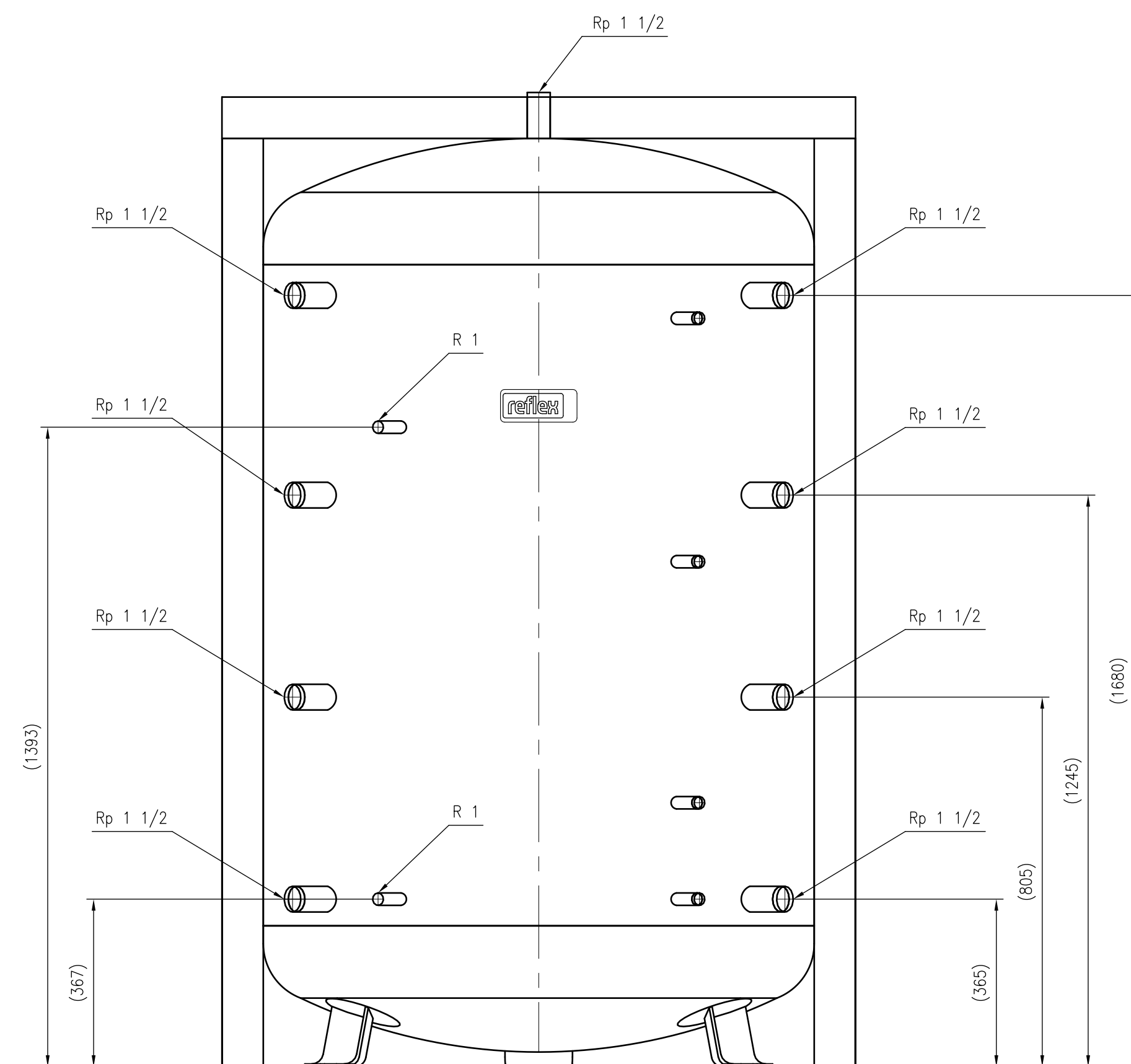
Front view
