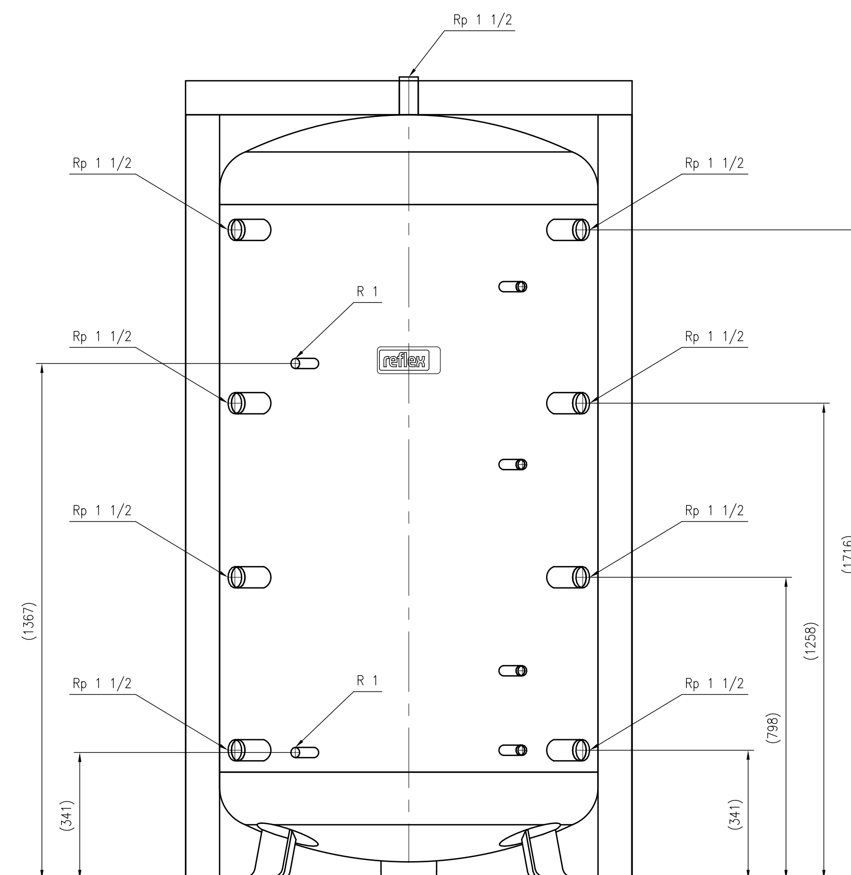
Front view
