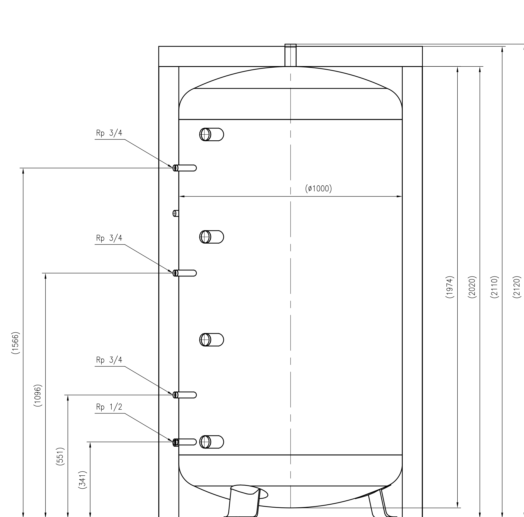
Side view
